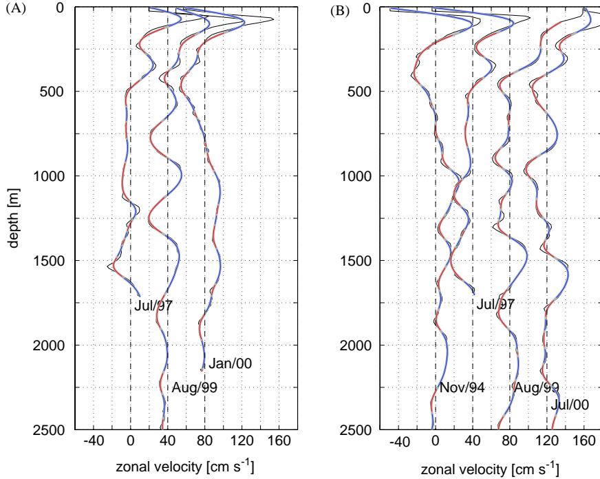
Fig. 4. Profiles of the zonal velocity on the equator at 23°W (A) and in 10–12.5°W (B) from observations with lowered ADCPs. The profiles are shifted by 40 \text{ cm s}^{-1} , and the zero velocity for each profile is shown as a dashed line. The smoothed profiles (thicker gray lines with red and blue overlaid) were obtained by applying a low-pass Butterworth filter with a cut-off length scale of 100 m. Red (blue) segments of the profiles indicate layers with positive (negative) curvatures, which are frequently associated with westward (eastward) jets.
