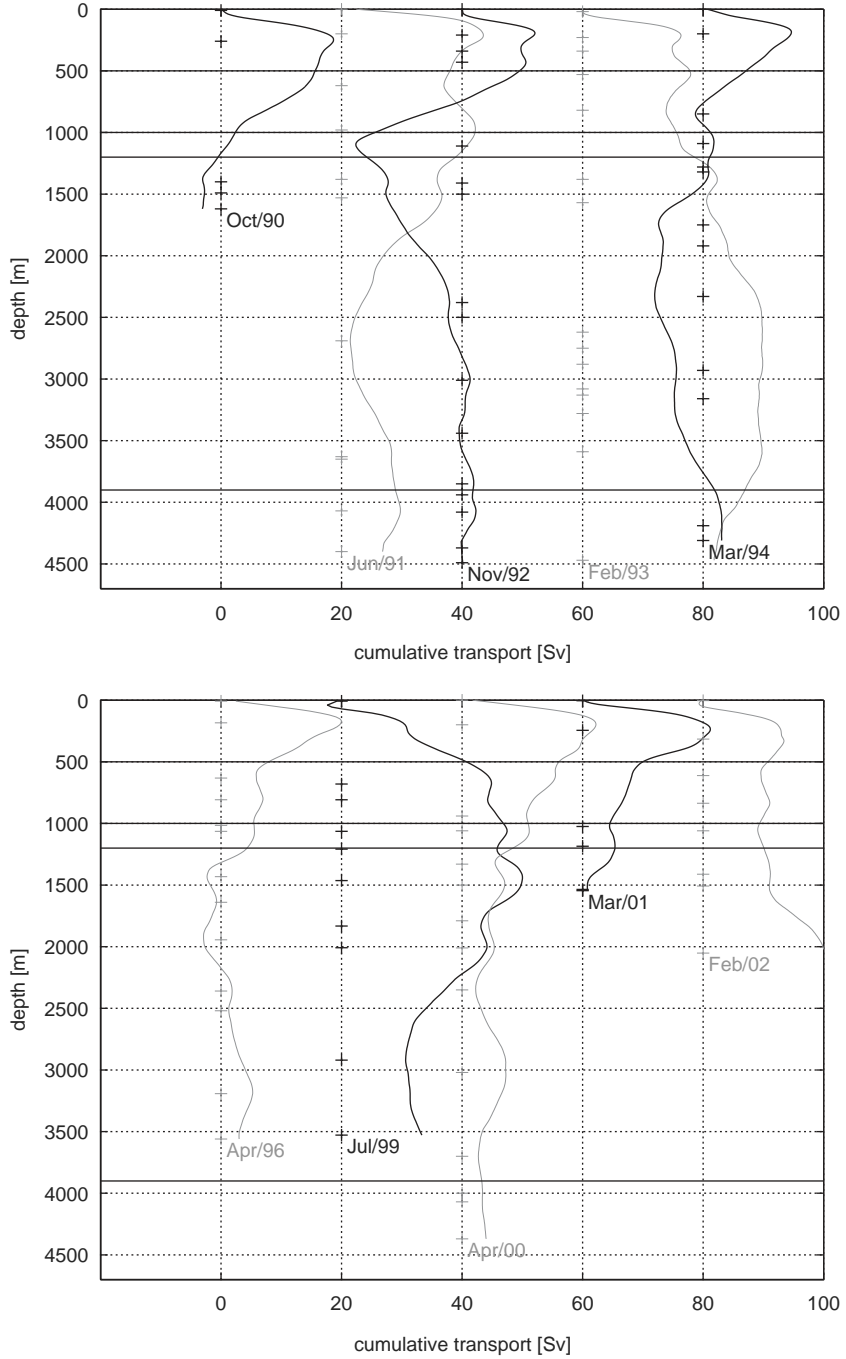
Fig. 6. Profiles of the zonal cumulative transport (integrated from top to bottom) at 35°W from observations with lowered ADCPs (Pegasus in February 1993). The profiles are shifted by 20 Sv ( 1 \text{ Sv} = 10^6 \text{ m}^3 \text{ s}^{-1} ). The crosses indicate the depths where the direction of the transport changes. The straight lines indicate the boundaries chosen for the Antarctic Intermediate Water (500–1000 m) and North Atlantic Deep Water (1200–3900 m) layer.
