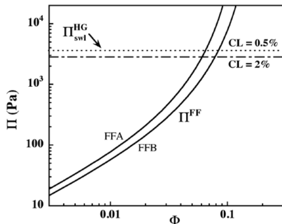
Figure 2 – Hydrogels : Initial swelling pressure \Pi_{\text{swl}}^{\text{HG}} at CL=0.5\% (horizontal dotted line) and at CL = 2\% (horizontal dashed-dotted line) (Table SI.1 of SI). Ferrofluids : Carnahan Starling adjustments of the osmotic pressure \Pi^{FF}(\Phi) of nanoparticles FFA and FFB following equ. (SI.7) – full lines (parameters : see table SI.2).
