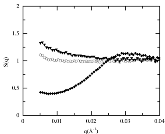
Figure 7 – Ferrogels at swelling equilibrium FGA - CL = 0.5% - Structure factor of the nanoparticles S(q) versus q at \Phi_{\text{equil}} = 0.5\% (solid triangles), 1.1% (open circles) and 3% (solid diamonds).
