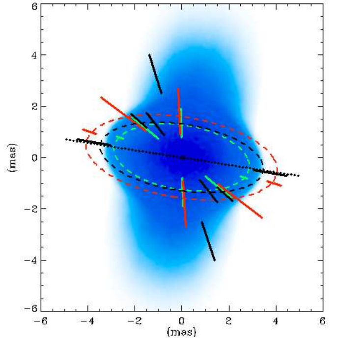
Fig. 4. \alpha Ara envelope at 8\ \mu\text{m} (green bars) and 12\ \mu\text{m} (red bars) assuming a uniform disk + an unresolved star model plotted as a function of baseline orientation. VLTI/AMBER measurements (black bars) are from Meilland et al. (2007a) and the corresponding best SIMECA model in the continuum (shaded background) are also shown. The black, green, and red ellipses correspond to the uniform ellipse fit of the equatorial disk presented in Table 6 at 2.1 , 8 , and 12\ \mu\text{m} , respectively. The orientation of the major axis (dotted black line) is perpendicular to polarization angle measurement obtained by Yudin & Evans (1998).
