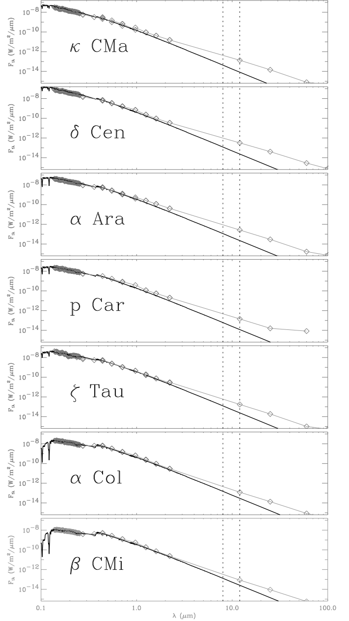
Fig. 2. Reconstructed SEDs for the 7 Be star systems observed with the VLT/MIDI instrument are shown with gray solid lines. Diamonds represent measurements taken from the VIZIER database. The portions of the SEDs up to 1\mu\text{m} (solid black lines) are fitted using reddened Kurucz models with the stellar parameters given in Table 4. Dashed lines represent the wavelengths for which the envelope flux is calculated, i.e., at 8\mu\text{m} , and 12\mu\text{m} .
