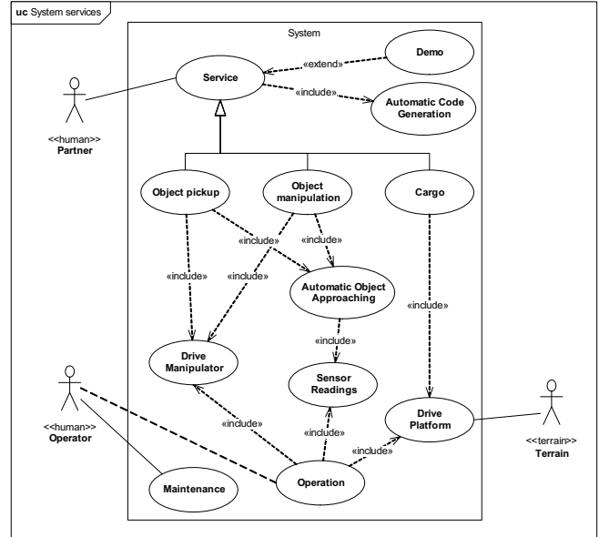
Figure 3 System services
