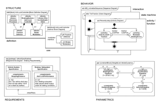
Figure 1 SysML pillars
