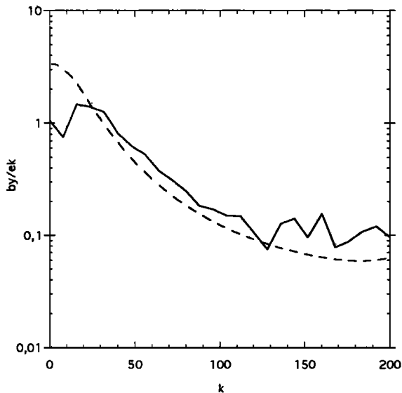
Figure 2. The ratio B_y/E_x in simulation units (the magnetic field is multiplied by the light velocity). A ratio equal to 1 represents electromagnetic waves with equal energy on the magnetic and on the electric components. The simulation results are plotted as a solid line, and the WHAMP results are plotted as a dashed line.
