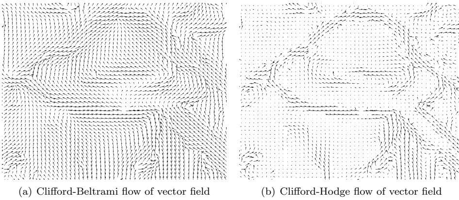
FIG. 4.3. Unit vector field of edge orientations regularization for h_i = 0.1
