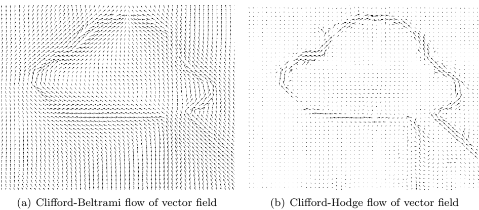
FIG. 4.4. Unit vector field of edge orientations regularization for h_i = 0.01
