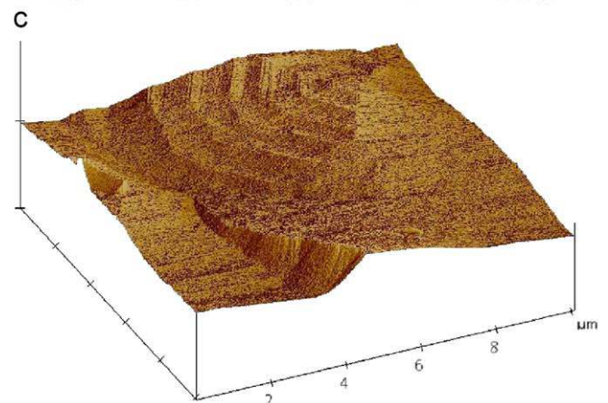
Fig. 10. SEM (a) and AFM ((b) and (c)) images of an AlN layer deposited at 1750^\circ\text{C} and 10\text{Torr} on 6H SiC (on axis).
