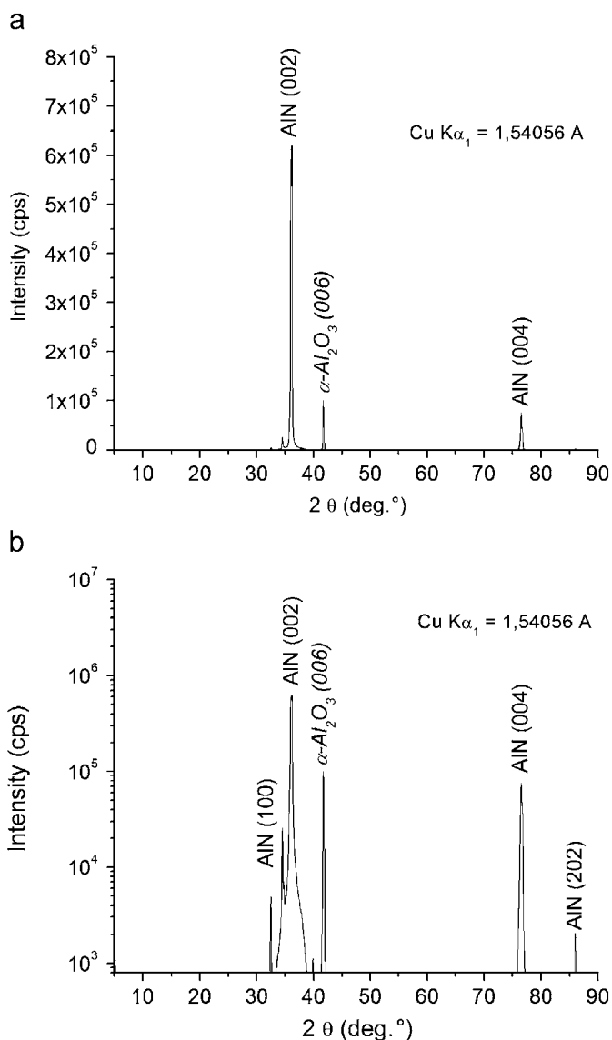
Fig. 7. Example of \theta/2\theta X-ray diffraction pattern of a 2H AlN layer deposited on (0001) \text{Al}_2\text{O}_3 single crystal substrate: (a) I = f(2\theta) and (b) \log(I) = f(2\theta) .
