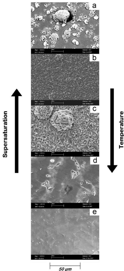
Fig. 9. SEM images of AlN layers grown on 4H SiC substrates at 1100^\circ\text{C} (a), 1300^\circ\text{C} (b), 1500^\circ\text{C} (c), 1650^\circ\text{C} (d) and 1750^\circ\text{C} (e) (constant reactants partial pressures and P = 10\text{Torr} ).
