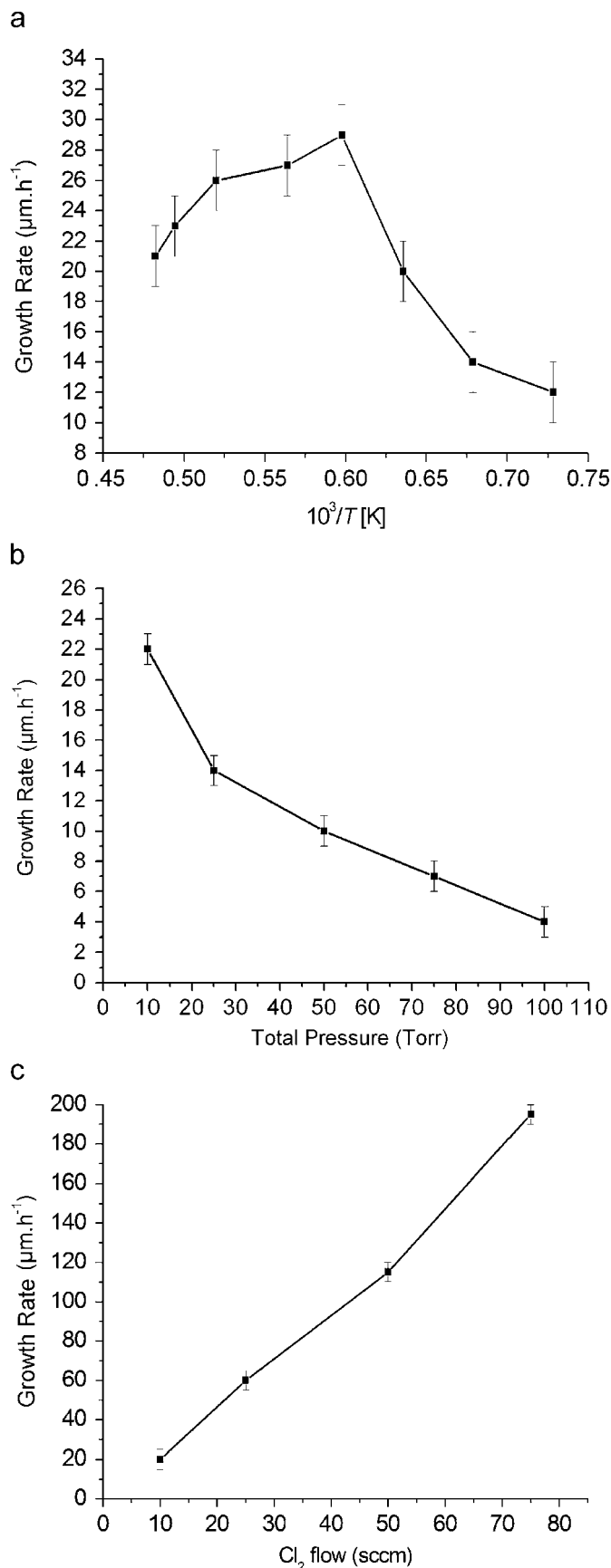
Fig. 6. Temperature (a), total pressure (b), and chlorine flow rate (c) effects on AlN growth rate on (0001) 4H SiC substrates.
