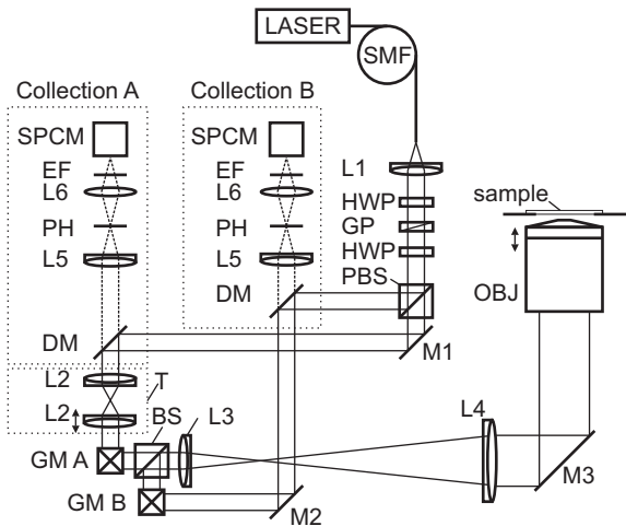
FIG. 1: Schematics of the dual spot FCS system. Abbreviations: SMF, single mode fiber; L1-L6, achromatic doublets ( L1 = 25 mm, L2 = 30 mm, L3 = 100 mm, L4 = 300 mm, L5 = 150 mm, L6 = 50 mm); HWP, half-wave plate; GP, Glan polarizer; PBS, polarizing beamsplitter; M1-M3, mirrors; DM, dichroic mirror; T, telescope; GM A (resp., B), galvanometric mirror set for channel A (resp., B); OBJ, water immersion microscope objective; PH, pinhole; EF, emission filter; SPCM: single photon counting module.
