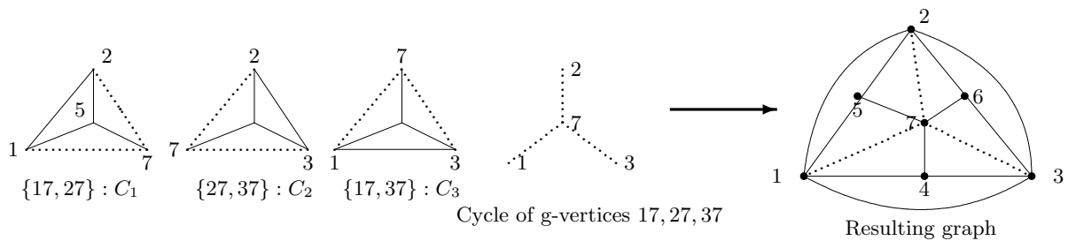
Fig. 3. Resulting graph is formed as 3-closure of path of 2-closures C_1 : \{2, 7\} : C_2 : \{3, 7\} : C_3 : \{1, 7\} : \dots . Actually, cycle of g-edges is \{17, 27\}, \{27, 37\}, \{37, 17\} , but we may in place of it considering corresponding cycle of g-vertices 17, 27, 37.
