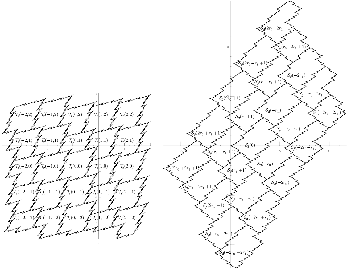
FIGURE 5. SRS tiles T_r(\mathbf{x}) associated with \mathbf{r} = (-1/\beta, -1/\beta^2) , \beta^3 = 3\beta^2 - 1 , (left) and the corresponding \beta -tiles \mathcal{R}_\beta(\{\mathbf{r}\mathbf{x}\}) = \mathcal{S}_\beta(\{\mathbf{r}\mathbf{x}\}) (right).
