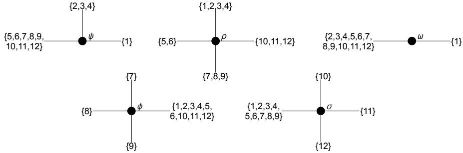
(c) The corresponding partial partitioning trees in \mathcal{P} .
