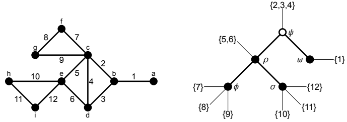
(a) A graph G = (V,E) . (b) A partial partitioning tree in \mathcal{P}^\dagger , with \psi as root. Here, the bag associated to node \psi (in the corresponding classical tree decomposition) would be \{b, c, d\} .
