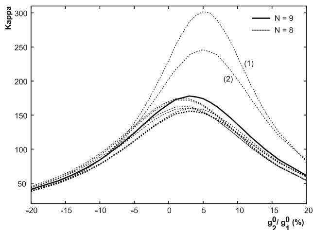
Figure 6. Fisher concentration parameter ( \kappa ) computed for the Oligocene poles represented in the Indo-Atlantic hot spot reference frame. The poles locations have been recalculated for various quadrupole ( g_2^0 )/dipole ( g_1^0 ) field ratio. The bold curve is computed for the nine selected poles listed in Table 2. The nine dashed curves are obtained for subset of eight poles, one different pole being removed in turn. Maximum values for \kappa are found for a quadrupole/dipole field ratio of 5% when the Principe volcanic pole (curve 1) or when the Liverpool volcano pole (curve 2) is removed.
