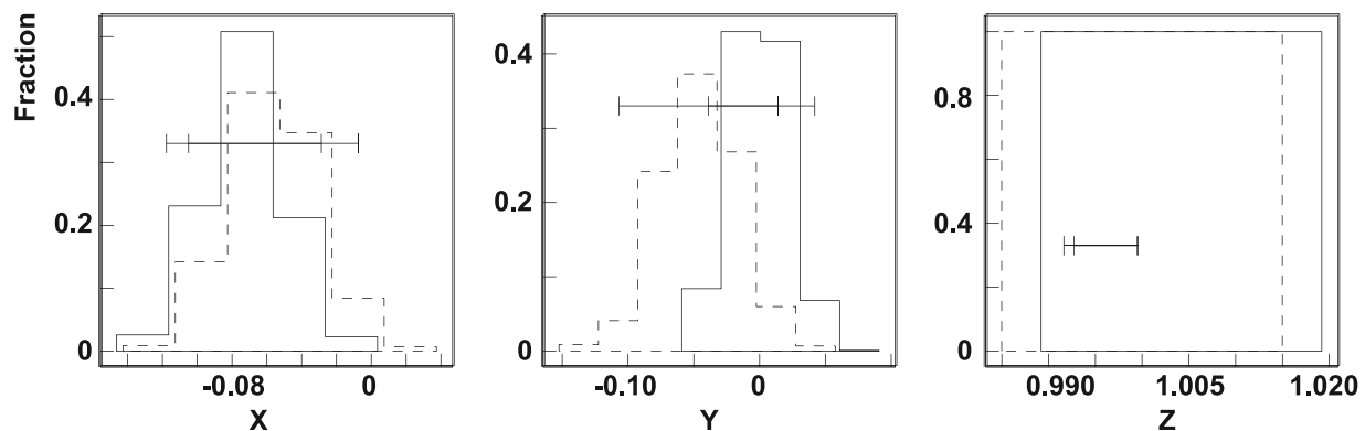
Figure 4. Histograms of Cartesian coordinates of the mean bootstrapped normal (solid line) and reverse (dashed line) VGP and their 95% confidence intervals [Tauxe, 1998] for the PSV data set (N = 233). In order to directly compare the two distributions, VGPs of reversed polarity have been flipped to their antipode. The two means cannot be distinguished at the 95% level of confidence since the confidence intervals for the two distributions overlap for each Cartesian coordinate.
