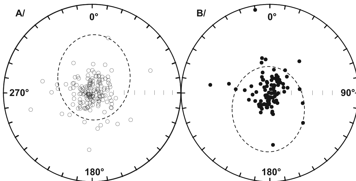
Figure 7. Whole data set ( N = 258 ) for the Kerguelen local field directions with (a) negative and (b) positive inclinations plotted on equal-area diagrams. For both diagrams the data have been rotated to the mean normal field direction calculated from the mean paleomagnetic pole. The dashed curves are the threshold for the inclinations and declinations, which give VGP location at an angular distance larger than 45^\circ from the mean pole axis.
