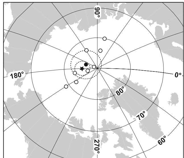
Figure 5. Selected paleomagnetic pole positions with respect to the Indo-Atlantic hot spot reference frame for the 25–30 Ma time interval (open circles) and their average (solid circle) compared with the Kerguelen pole (solid star). Dashed curves are the 95% confidence limit for the mean poles calculated assuming a Fisherian distribution.
