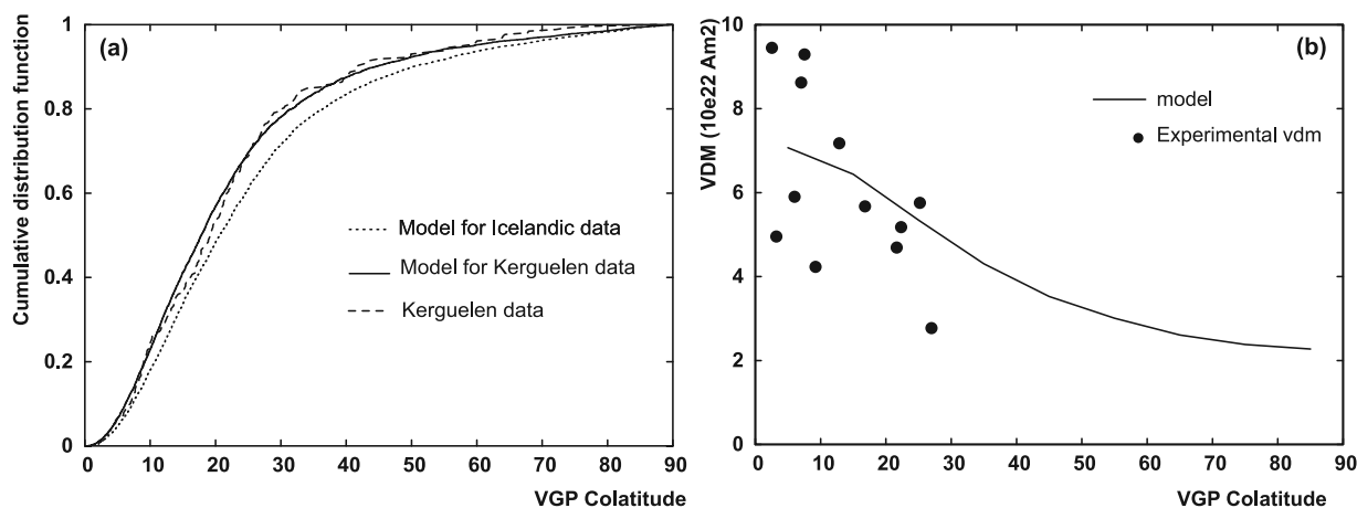
Figure 9. Data and Camps and Prévot's [1996] statistical model for the Kerguelen data set. The model is adjusted from the VGP colatitudes only, using the parameter \sigma_{AD}^2 = 0.2 , \sigma_{SV}^2 = 0.029 (see Camps and Prévot [1996] for a detailed description of the model). (a) Cumulative distribution for the VGP colatitudes, VGPs of reverse polarity being flipped to their antipodes. (b) Comparison of VDMs (solid circles) obtained for Kerguelen lava flows [ Plenier et al. , 2003] to the model outcomes, assuming in the model a value of 7 \times 10^{22} A m 2 for the mean axial dipole moment. This value corresponds to the mean experimental VDM for VGPs of colatitude lower than 10°.
