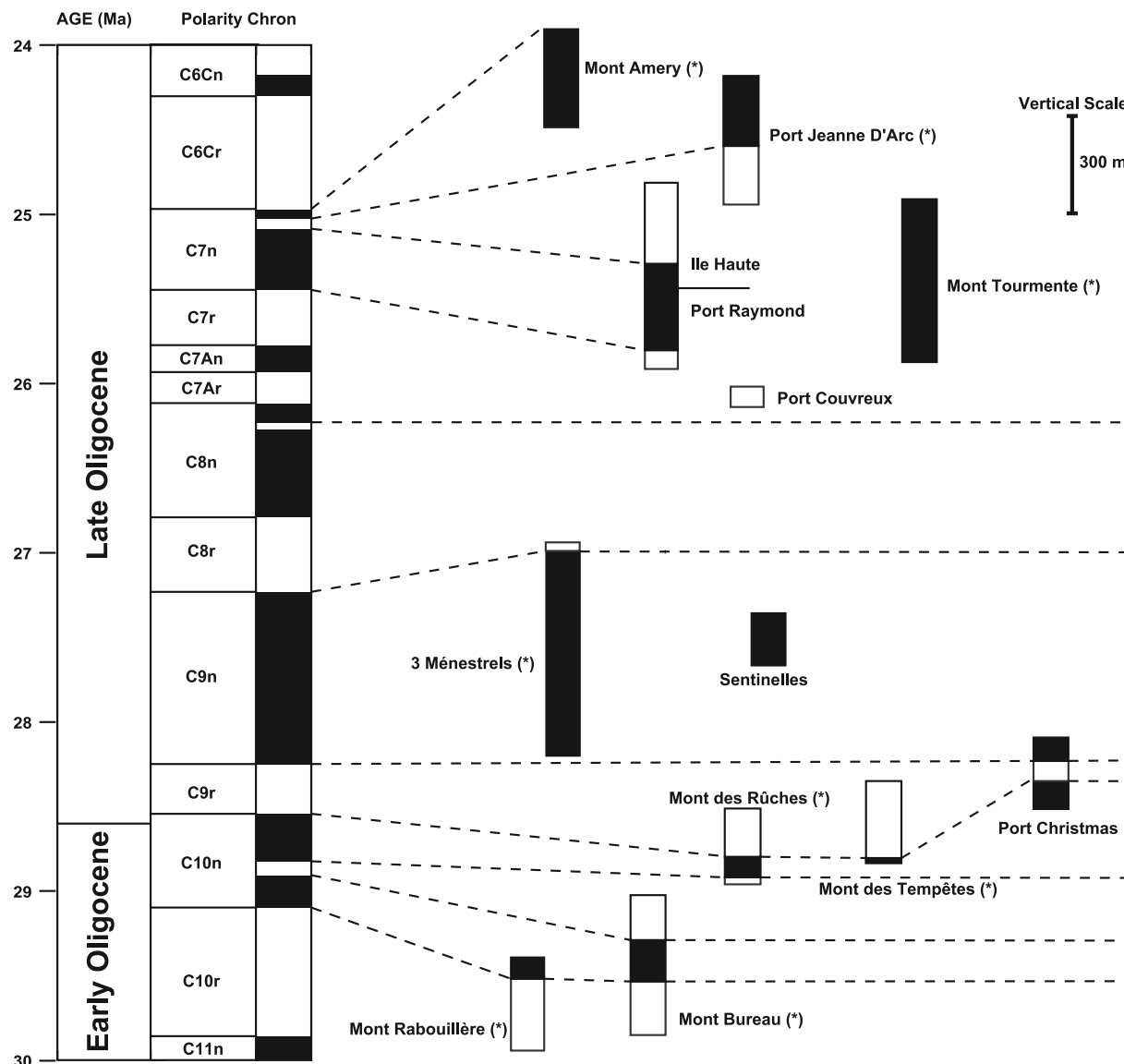
Figure 3. Magnetostratigraphic correlations with the global geomagnetic polarity timescale [Huestis and Acton, 1997]. The sections for which radiometric ages are available are marked with an asterisk. We used geological and geochemical observations to correlate the remaining sections.
