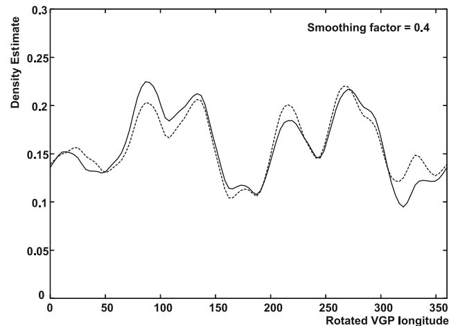
Figure 8. Nonparametric density estimates calculated by means of a quartic kernel function for VGP longitude rotated in the paleomagnetic pole ( \lambda = 85.5^\circ , \phi = 189.3^\circ ) reference frame for the whole data set N = 258 (solid curve) and the PSV data set N = 233 (dashed curve).
