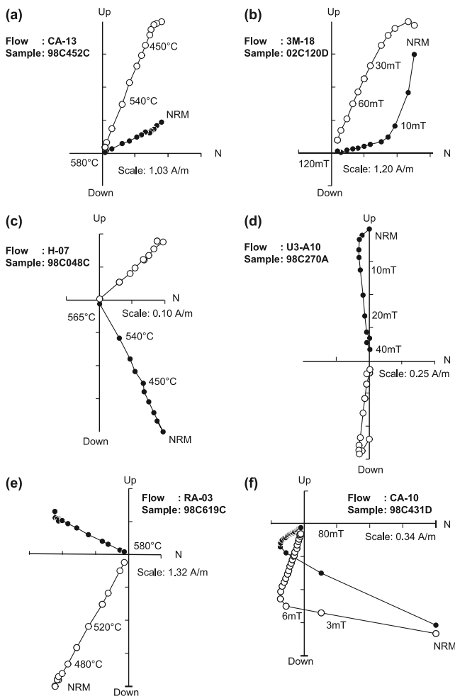
Figure 2. Example of vector endpoint diagrams of (left) progressive thermal and (right) AF demagnetizations for (a, b) normal, (c, d) intermediate, and (e, f) reverse directions. Projections are in geographic coordinates for Figures 2a, 2c, 2e, and 2f or tilt-corrected coordinates for Figures 2b and 2d. Solid (open) symbols represent projection into horizontal (vertical) planes. Figures 2b, 2d, and 2f show that the ChRM are easily isolated even when large secondary components are present.
