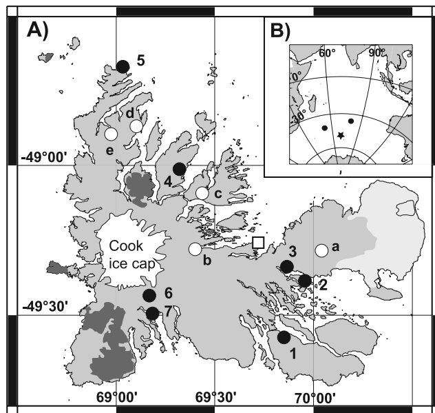
Figure 1. (a) Location of the sampling sites on a Kerguelen Archipelago map. The numbered solid circles (this study) are 1, Port Jeanne d'Arc; 2, Ile Haute; 3, Port Raymond; 4, Mont Bureau; 5, Port Christmas; 6, Trois Ménéstrels; and 7, Sentinelles. The lettered open circles [ Plenier et al. , 2002] are a, Mont Amery; b, Mont Tourmente; c, Mont Rabouillère; d, Mont Tempête; and e, Mont des Ruches. The open square is Port Couvreur [ Henry and Plessard , 1997]. The distributions of quaternary deposits (light grey), flood basalts (medium grey), and plutonic complexes (dark grey) are also shown. (b) Location in the Indian Ocean of the Kerguelen Archipelago (solid star) and the Crozet Archipelago and New Amsterdam (solid circles).
