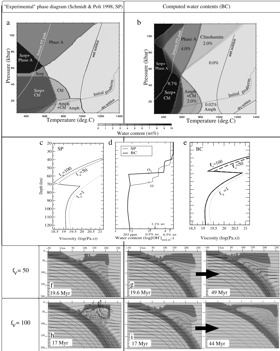
Figure 12. Influence of peridotite mineralogy on the subduction erosion process. (a and b) Water content grid as a function of T and P for lherzolitic compositions and water-saturated conditions, obtained by experimental approach (Figure 12a, Schmidt and Poli [1998], SP) and/or by a thermodynamic calculation (Figure 12b, this study, BC). (d) Water content profiles across the lithosphere for the initial geotherm and the two water content grids. (c and e) Reference viscosity profiles, computed with \dot{\epsilon}_{ref} = 10^{-14} \text{ s}^{-1} , using the initial geotherm and the water content profiles for grid SP (Figure 12c) and grid BC (Figure 12e). (f and h) Subduction simulations for grid SP. (g and i) Subduction simulations for grid BC. Note the gray color scale indicating water content is the same as in Figure 4.
