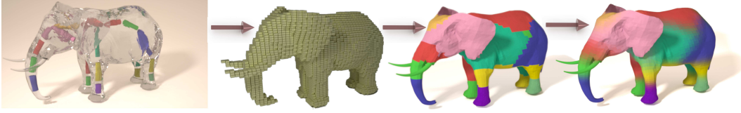
Figure 6: Complete pipe-line of skinning weights computation. Left: Initial mesh + skeleton. Second picture: Voxelized domain bounded by the mesh. Third picture: Color encoded result after volumetric distance propagation (only the main influencing bone is shown). Right: Final result after surfacic diffusion.
