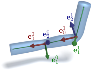
Figure 4: Local frames defined for a articulated cylinder deformed by smooth skinning using three segments.
