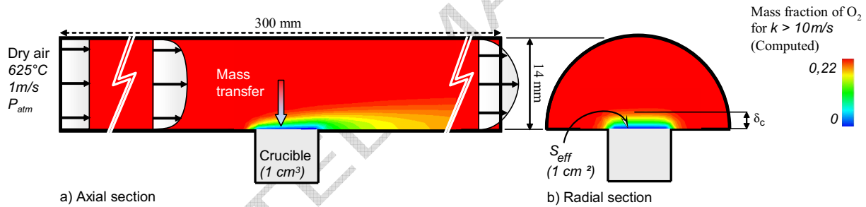
Fig. 1. Oxidation reactor geometry and experimental conditions (dry air, T = 898\text{ K} , P = 1\text{ atm} ).
