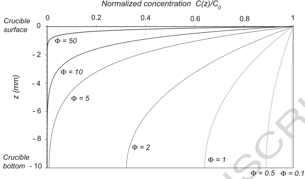
Fig. 5. Normalized concentration gradient in a fiber bundle as a function of \Phi .
