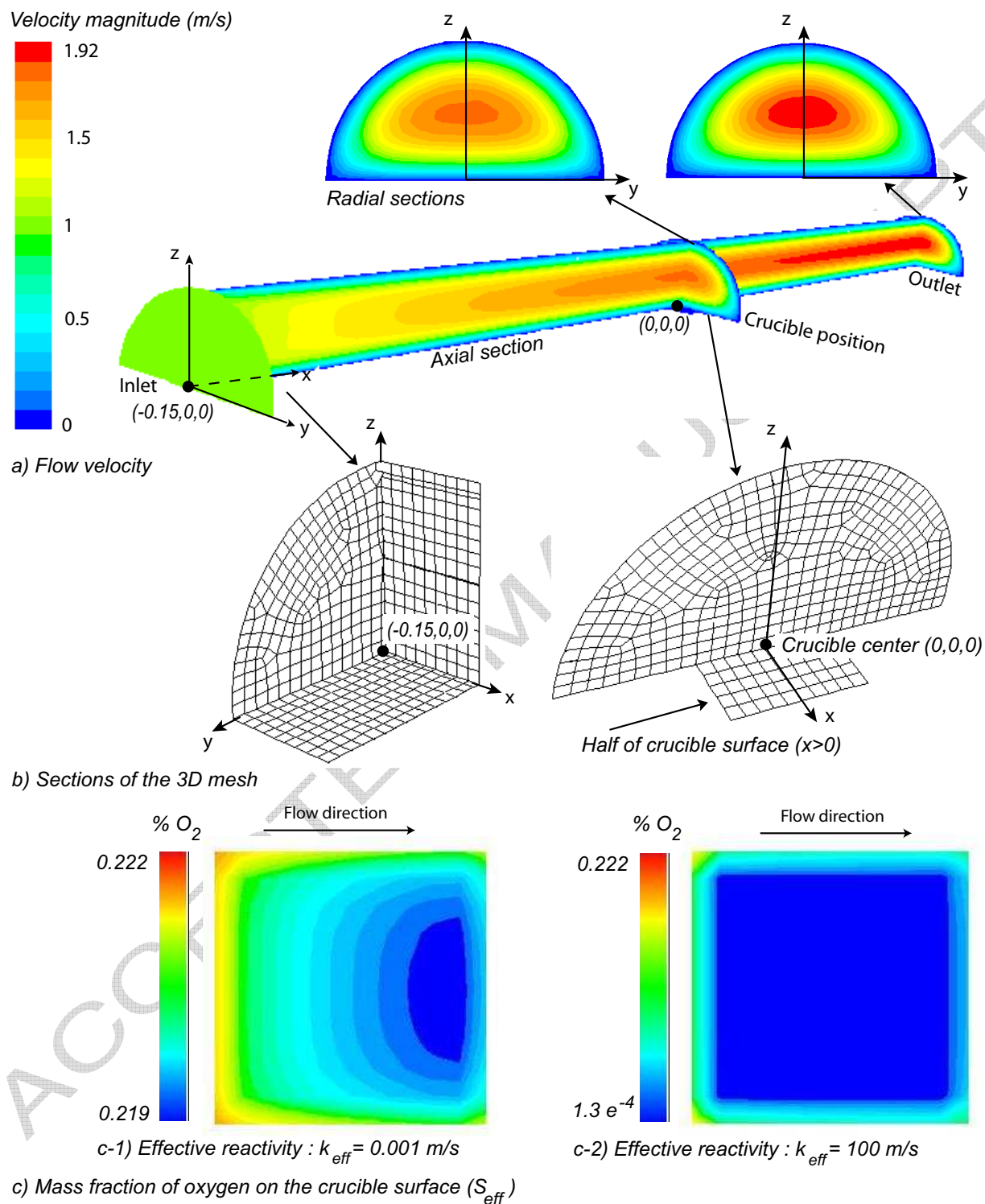
Fig. 3. 3D numerical simulation results
