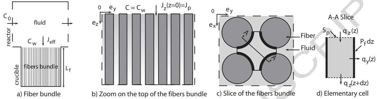
Fig. 2. Sketch of a unidirectional bundle of cylindrical fibers placed in a crucible
