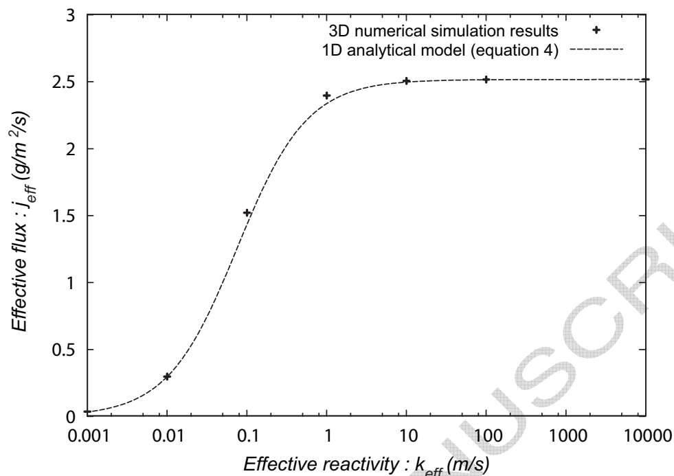
Fig. 4. Effective flux as a function of effective reactivity : comparison of 1D analytical and 3D numerical results.
