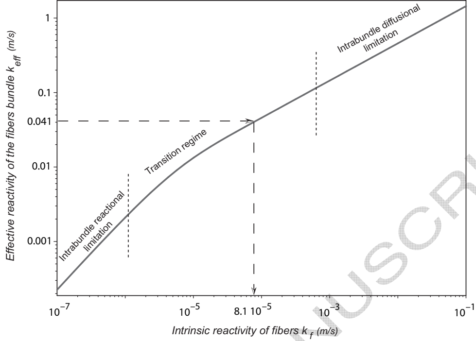
Fig. 6. Illustration of a plot of k_{eff} versus k_f for the fiber bundle F4 - R
