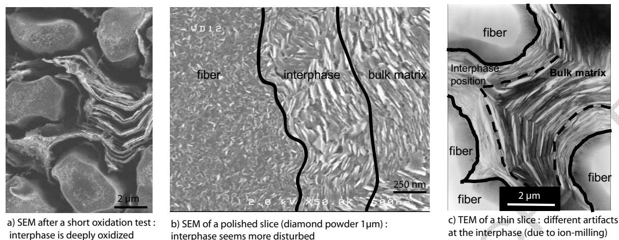
Fig. 7. Observation of the interphase lying between fibers and inter-yarn matrix (3D C/C)
