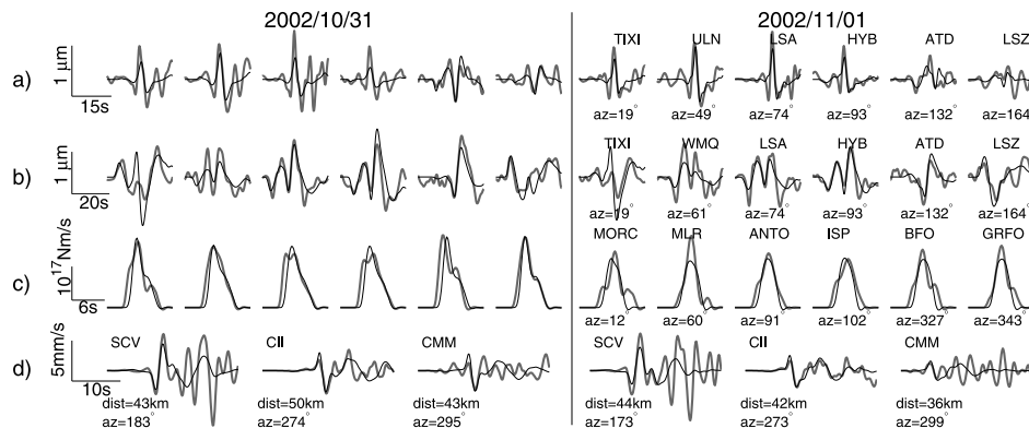
Figure 2. Agreement between data and synthetics (both lowpass filtered at 0.5 Hz) for representative stations. Waveforms relative to the MS1 are on the left and these of MS2 on the right. (a) P waves. (b) SH waves. (c) RSTFs deduced from the EGF analysis. (d) Local data; CMM station is presented but was not used to define the inverse model. Data are represented by thick gray lines whereas synthetics corresponding to the source models of Figure 3 are thin black lines. Selected stations and scales are the same for both shocks. Names and azimuths of stations are written on the right for the MS2 but, for clarity, have not been repeated for MS1. Agreement between data and synthetics at all stations can be seen in Figure A1.
