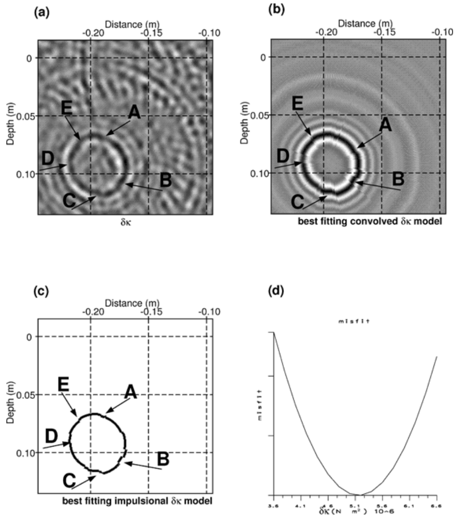
Figure 12. Inversion for the PVC cylinder. Results of the post-processing sequence applied to the tomographic model \delta\kappa in (a). (b) Best-fitting convolved model. (c) Best-fitting impulsional model representing the geometry and dimensions of the hollow PVC cylinder. (d) Misfit for \delta\kappa .
