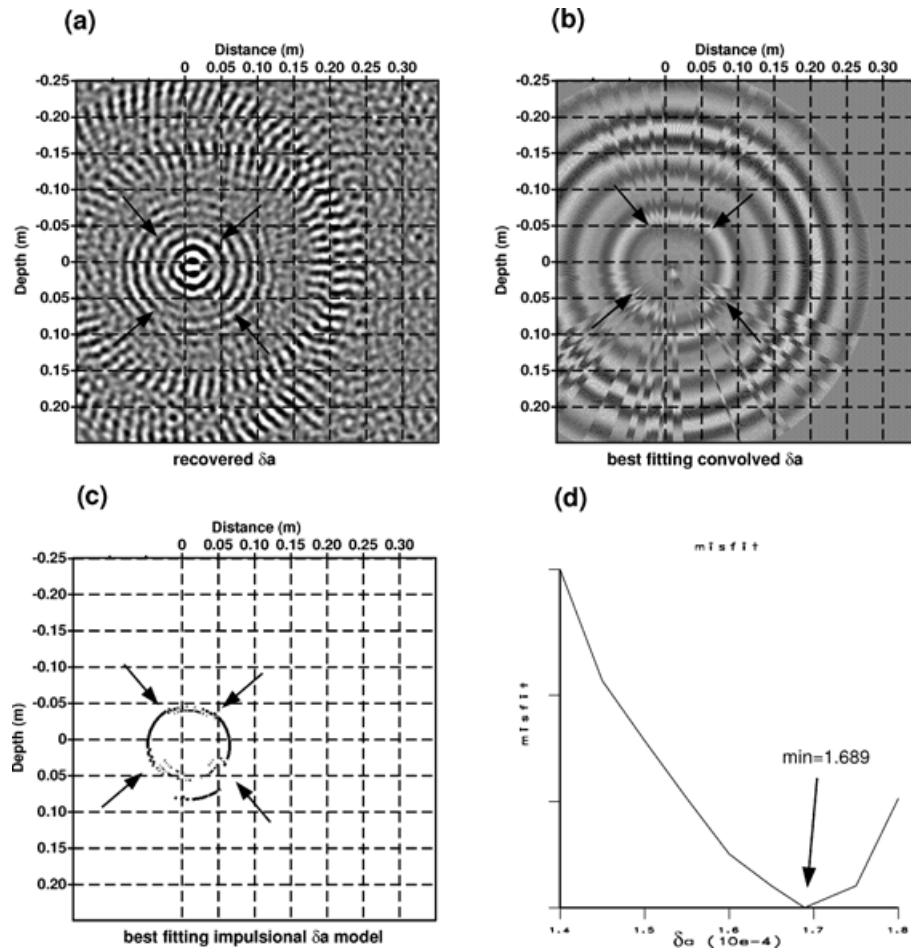
Figure 15. Inversion for the lava sample. (a) Tomographic model for \delta a . (b) The best-fitting convolved model from the post-processing sequence applied to (a). (c) The best-fitting impulsive model. (d) The misfit function representing the perturbations of \delta a and the minimum.
