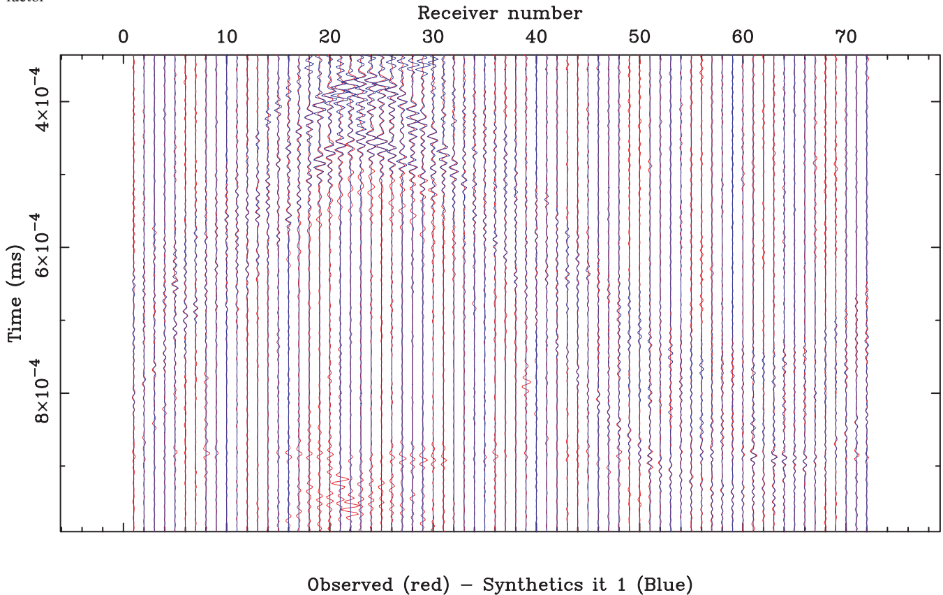
Figure 9. Comparison of recorded and synthetic traces obtained in three-parameter inversion.
