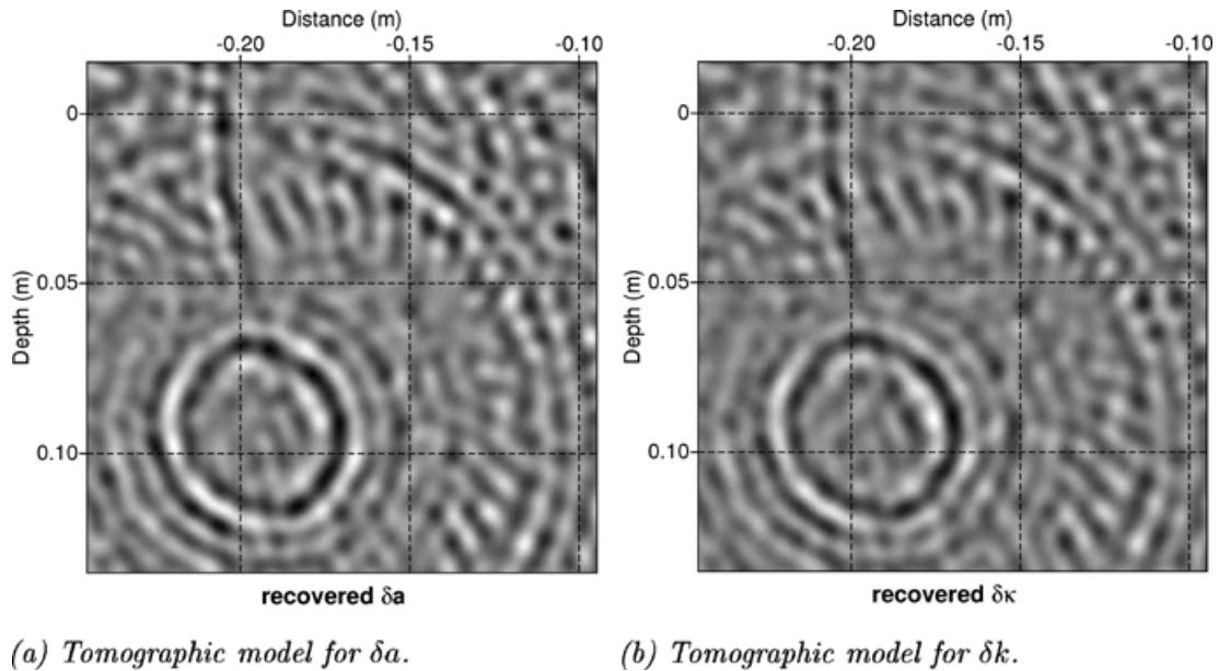
Figure 6. Recovered \delta a and \delta \kappa sections for the PVC cylinder after one iteration for an assumed value of \alpha = 0.5 . The shape of the cylinder is clearly identifiable on both sections notwithstanding a contamination by the source signature and multiples.
