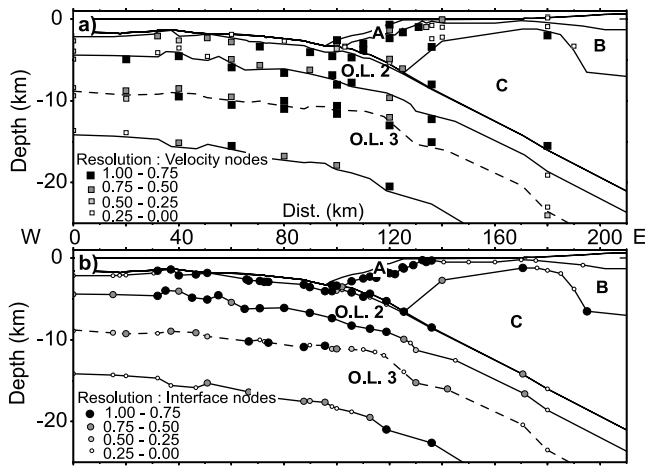
Figure 3. Resolution values calculated from the travel time inversion of the final velocity model: resolution values of the velocity nodes (a), and resolution values of the interface nodes (b).
