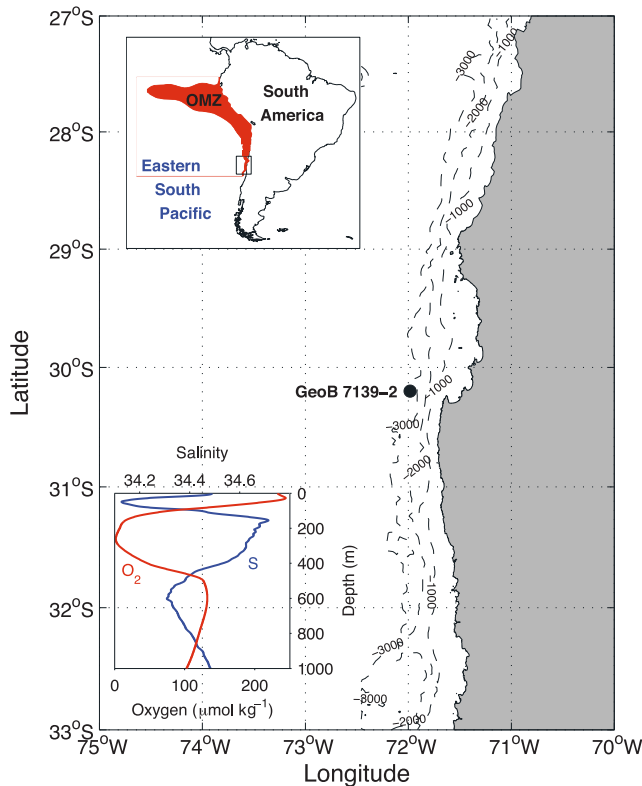
Figure 1. Map of central to northern Chile and the adjacent eastern South Pacific showing the location of the sediment core GeoB 7139-2 (30°12.00'S; 71°58.99'W; 3267 m water depth). Dashed lines represent the 1000, 2000, and 3000 m isobaths. The core site lies at the southern boundary of the region where O 2 levels drop below 20 μM as an annual mean (red shaded area in the upper inset). The lower inset shows salinity (solid blue line) and oxygen (solid red line) distributions as a function of water depth at the core site. Note the oxygen-depleted waters (oxygen minimum zone (OMZ)) between 150 and 350 m and the salinity minimum at ~100 m.
