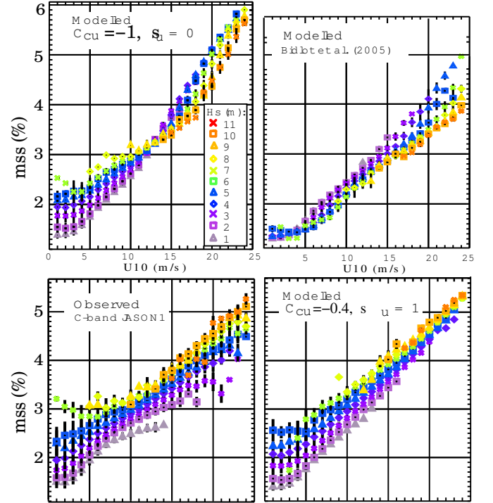
FIG. 8. Variation of the surface mean square slope estimated as either 0.64/\sigma_0 using the C-band altimeter on board JASON-1, after the correction of a 1.2 dB bias in the JASON data, or by integration of modelled spectra from 0 to 0.72 Hz, with either the C_{cu} = -0.4 and s_u = 1 parameterization (TEST441) or the parameterization by BAJ. For modelled values a constant 0.011 is added to account for the short waves that contribute to the satellite signal and that are not resolved in the model. This saturated high frequency tail is consistent with the observations of Vandemark et al. (2004). The original 1 Hz data from JASON is subsampled at 0.5 Hz and averaged over 10 s, namely 58 km along the satellite track. The same averaging is applied to the wave model result, giving the 393382 observations reported here, for the first half year of 2007.
