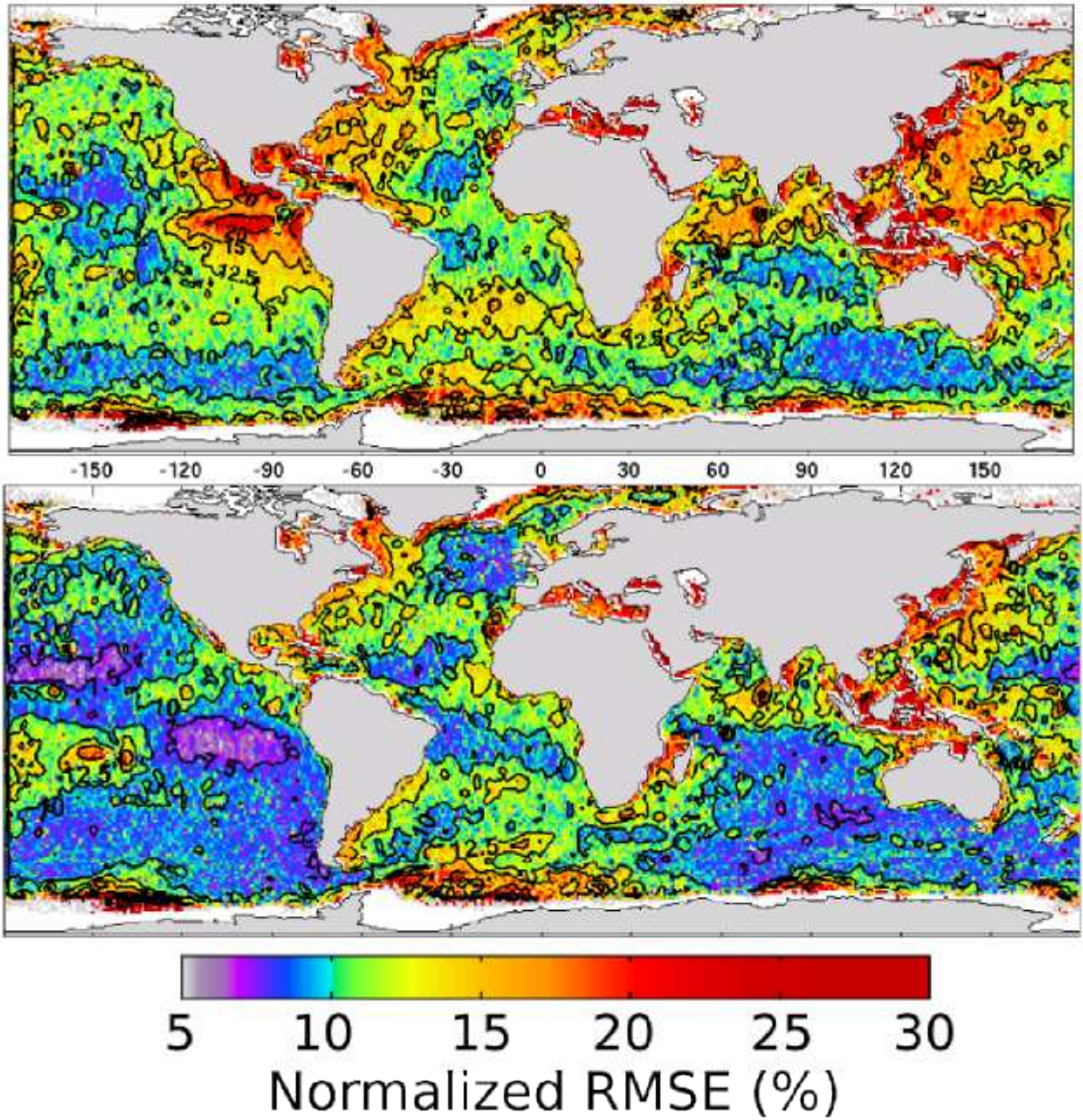
FIG. 11. Normalized RMSE for the significant wave height over the year 2007, in percents. The global 0.5^\circ resolution WWATCH model is compared to altimeters JASON, ENVISAT and GFO following the method of Raschle et al. (2008). The top panel is the result with the BAJ parameterization, and the bottom panel is the result with the C_{cu} = -0.4 and s_u = 1 (TEST441) parameterization.
