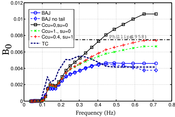
FIG. 6. Values of the spectral saturation B_0 for the cases presented in figure 5.
