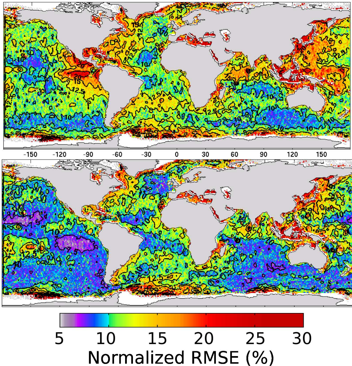
FIG. 11. Normalized RMSE for the year 2007 in percents. The global 0.5 WWATCH model is compared to altimeters JASON, ENVISAT and GFO following the method of Raschle et al. (2008). The top panel is the result with the BAJ parameterization, and the bottom panel is the result with the C_{cu} = 0.4 and s_u = 1 (TEST441) parameterization.
