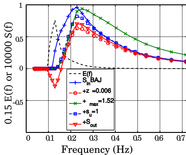
FIG. 7. Incremental adjustments to the wind-wave interaction source term S_{atm} , going from the BAJ form to the one used in TEST441. The effect of modifying a new parameter are clearly seen. The reduction of z_\alpha from 0.011 to 0.006 strongly reduces the low frequency input, which is probably overestimated in BAJ when average (20%) levels of gustiness are considered: now the wind input goes to zero for f = 0.13 , which corresponds to C/U_{10} = 0.83 , whereas it is still significant at that wave age in the BAJ parameterization. As a result the much lower input level need a readjustment, but increasing \beta_{max} to 1.52. Yet, this high value of \beta_{max} produces very high wind stress values and thus a very strong high frequency input. This is where the sheltering term s_u = 1 allows a decent balance at high frequency. Finally, the addition of the air-sea friction term that gives swell dissipation produces a significant reduction of the input to the wind sea at f = 0.25 Hz. It is questionable whether this mechanism also applies in the presence of the critical layer for those waves. This matter clearly requires more theoretical and experimental investigation.
