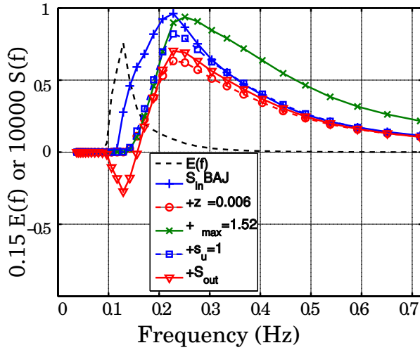
FIG. 7. Incremental adjustments to the wind-wave interaction source term S_{\text{atm}} , going from the BAJ form to the one used in TEST441. The effect of modifying a new parameter are clearly seen. The reduction of z_\alpha from 0.011 to 0.006 strongly reduces the low frequency input, which is probably overestimated in BAJ when average (20%) levels of gustiness are considered: now the wind input goes to zero for f = 0.13 , which corresponds to C/U_{10} = 0.83 , whereas it is still significant at that wave age in the BAJ parameterization. As a result the much lower input level need a readjustment, but increasing \beta_{\text{max}} to 1.52. Yet, this high value of \beta_{\text{max}} produces very high wind stress values and thus a very strong high frequency input. This is where the sheltering term s_u = 1 allows a decent balance at high frequency. Finally, the addition of the air-sea friction term that gives swell dissipation produces a significant reduction of the input to the wind sea at f = 0.25 Hz. It is questionable whether this mechanism also applies in the presence of the critical layer for those waves. This matter clearly requires more theoretical and experimental investigation.
