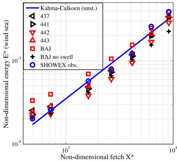
FIG. 3. Fetch-limited growth of the windsea energy in as a function of fetch on 3 November 1999, averaged over the time window 1200-1700 EST, from observations and model runs, with different model parameterizations (symbols): BAJ stands for Bidlot et al. (2007a). This figure is analogue to the figure 8 in Ardhuin et al. (2007), the model forcing and setting are identical. All parameters for BAJ, TEST441 and TEST443 are listed in tables A1 and A2. Input parameters for TEST443 are identical to those for TEST441, and TEST442 differs from TEST441 only in its isotropic direct breaking term, given by sB = 0 , \Delta_\theta = 180^\circ , and B_r = 0.0012 .
