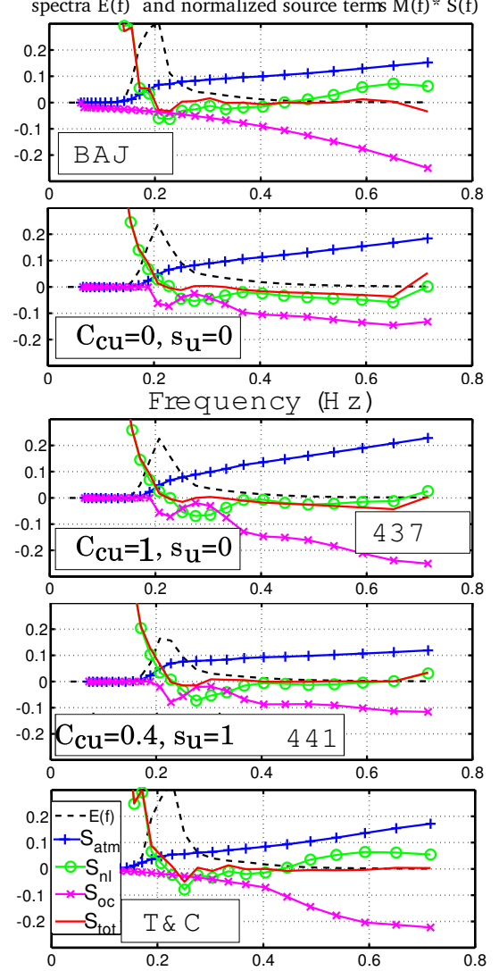
FIG. 4. Academic test case over a uniform ocean with a uniform 10 \text{ m s}^{-1} wind starting from rest, after 8 hours of integration, when C_p/U_{10} \approx 1 . Source term balances given by the parameterization BAJ, and the parameterizations proposed here with the successive introduction of the cumulative breaking and the wind sheltering effects with the parameters C_{cu} and s_u . For BAJ, a diagnostic f^{-5} tail is applied above 2.5 the mean frequency. In order to make the high frequency balance visible, the source terms are multiplied by the normalization function M(f) = \rho_w C / (\rho_a E(f) \sigma U_{10}) . The result with the parameterization of Tolman and Chalikov (1996) is also given for reference.
