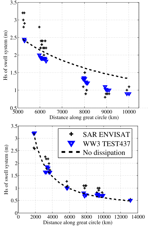
FIG. 1. Comparison of modelled swell significant heights, following the propagation of the two swells shown by Ardhuin et al. (2009) with peak periods of 15 s and high and low dissipation rates. Known biases in the level 2 data have been corrected following Collard et al. (2009).
