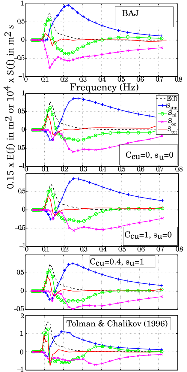
FIG. 5. Same as figure (4) but after 48 h of integration and without normalization of the source terms. Source term balances given by the parameterization BAJ, and the parameterizations proposed here with the successive introduction of the cumulative breaking and the wind sheltering effects with the parameters C_{cu} and s_u . For BAJ, a diagnostic f^{-5} tail is applied above 2.5 the mean frequency.
