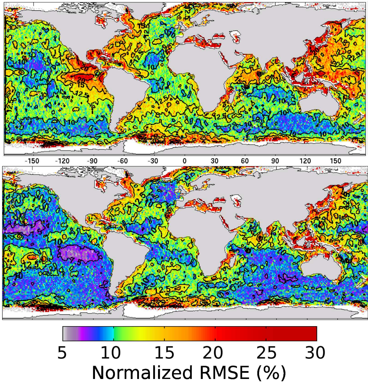
FIG. 11. Normalized RMSE for the year 2007 in percents. The global 0.5 WWATCH model is compared to altimeters JASON, ENVISAT and GFO following the method of Rascle et al. (2008). The top panel is the result with the BAJ parameterization, and the bottom panel is the result with the C_{cu} = 0.4 and s_u = 1 (TEST441) parameterization.
