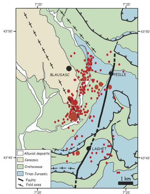
Figure 4. Simplified geological map of the Blausasc area [modified from Gèze et al. , 1968]. The epicentre alignment is located 2.5 km west of the Peille-Laghét fault above the Paillon valley.
