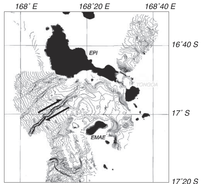
Figure 9. Multibeam bathymetry of part of the Sheppard area at the southern termination of the Back Arc Thrust Belt. Contour interval is 50 m. Data were acquired during the CALVA cruise [Eissen et al., 1997]. Arrows indicate present shearing motion in the Sheppard area as derived from Euler poles for the southern and central segments.
