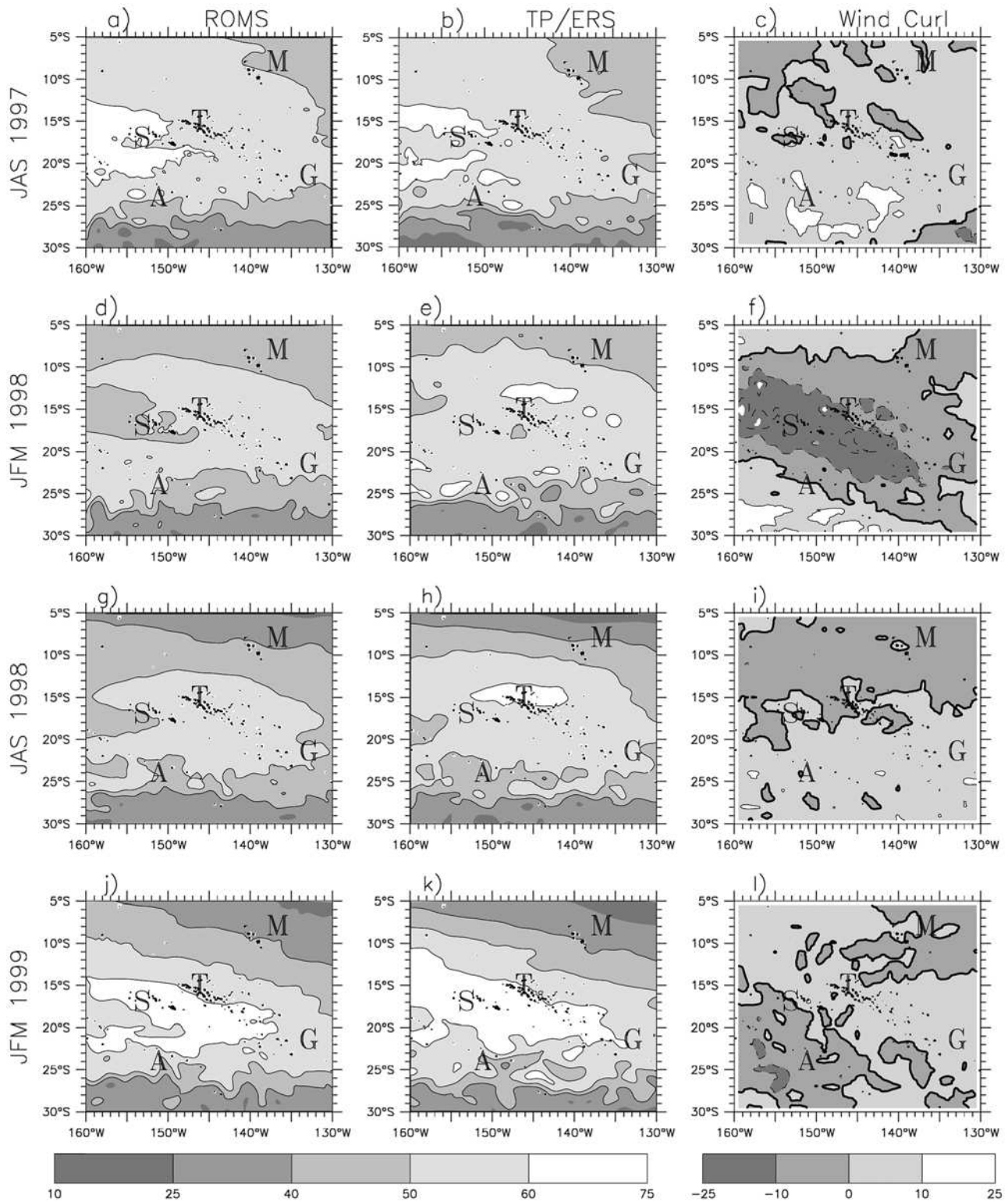
Figure 10. (left) Three-month average original ROMS SSH (in centimeters), (middle) TP/ERS SSH (in centimeters), and (right) satellite-derived wind curl ( 10^{-8} \text{ N m}^{-3} ) during (a–c) El Niño in winter 1997, (d–f) El Niño in summer 1998, and La Niña in (g–i) winter 1998 and (j–l) summer 1999. Contours are drawn every 10 cm for the SSH and every 1 \cdot 10^{-8} \text{ N m}^{-3} for the wind curl.
