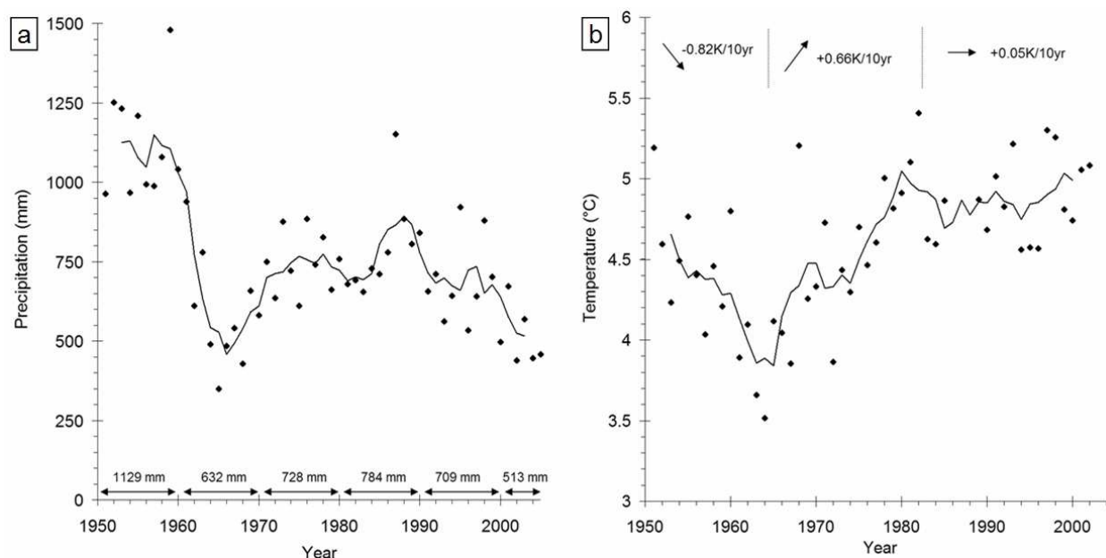
Figure 10: Temperature and precipitation at Port-aux-Français (80 km east of Cook ice cap). The symbols correspond to the yearly values whereas the lines are the 5-year running means. (a) Annual precipitation between 1951 and 2005. The decadal means of precipitation are given above the X-axis. (b) Mean annual temperature between 1951 and 2002. The temperature record has been split into three time periods for which the linear trend is given in the upper part of the graph.
