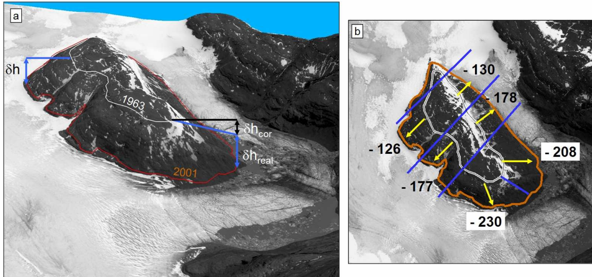
Figure 7: Growing nunataks as indicators of ice elevation changes. (a) 3D view of nunatak Lapparent (region of Ampère glacier, Figure 3) with its outline in 1963 (white) and 2001 (red). The blue arrows symbolize the thinning that can be measured using a single topography (here, SRTM). In the lowest parts of the nunatak, real elevation changes (noted \delta h_{real} ) were obtained after applying a \sim 50 m correction (symbolized by a black arrow and noted \delta h_{cor} ) to take into account the non horizontal slope of the 1963 ice surface. (b) Mean ice elevation changes around nunatak Lapparent between 1963 and 2000.
