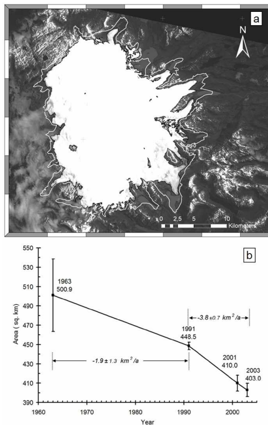
Figure 2: Retreat of Cook ice cap between 1963 and 2001. (a) 2001 Landsat image with the 1963 (white) and 2001 (black) glacier outlines. (b) Temporal changes of the ice-covered area. The rates of glacier shrinkage (km 2 /yr) are indicated for 1963-1991 and 1991-2003.
