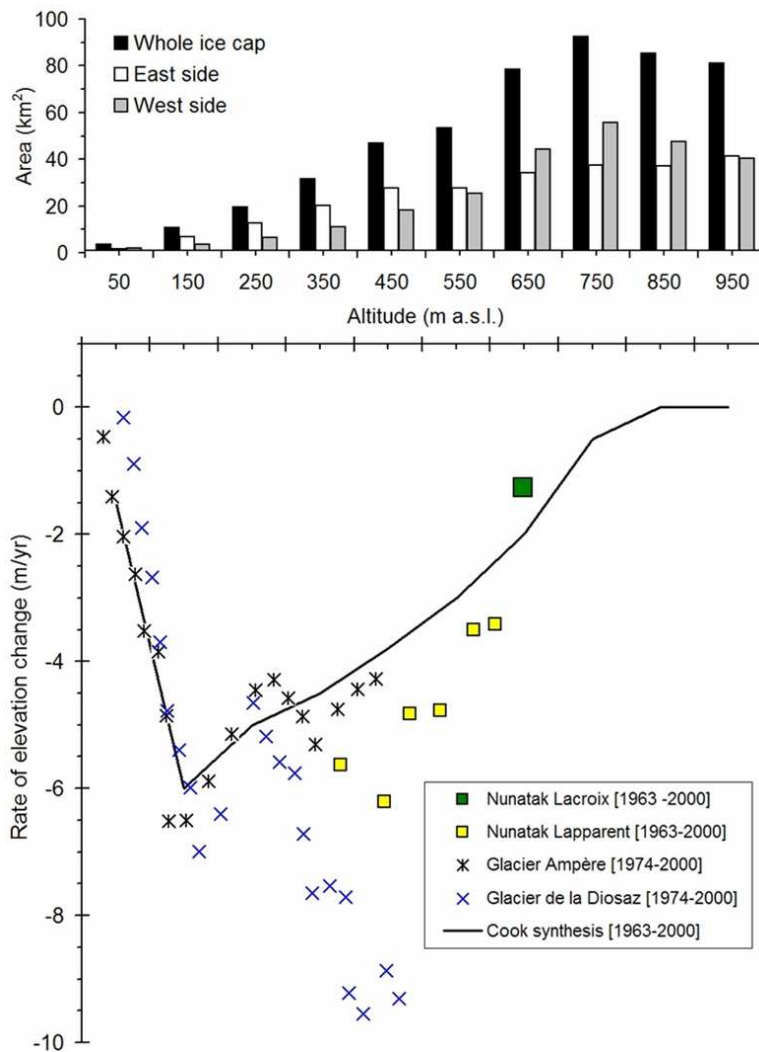
Figure 9: Hypsometry of Cook ice cap in 1963 (upper panel) and elevation changes as a function of altitude on different regions of the ice cap (lower panel). The elevation differences were measured by comparing two topographies (1974-2000, Figure 6) and analyzing the growth of nunataks (1963-2000, Figure 7).
