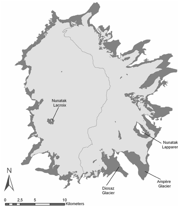
Figure 3: East/west asymmetry of Cook ice cap shrinkage. The dark grey represents ice-covered areas that disappeared between 1963 and 2001.
