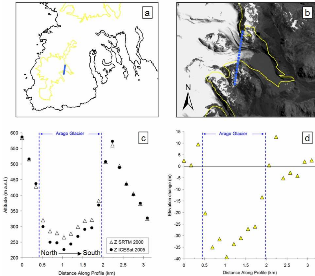
Figure 8. Recent (2000–2005) elevation changes on Rallier du Baty Peninsula (Figure 1). (a) Location of the 25 February 2005 ICESat track (laser period 3B) across Arago glacier; in yellow, the glacier limit in 1964; (b) close-up, background is a 2001 Landsat image; (c) elevation profile extracted from the SRTM DEM and ICESat; (d) elevation changes between February 2000 and February 2005.
