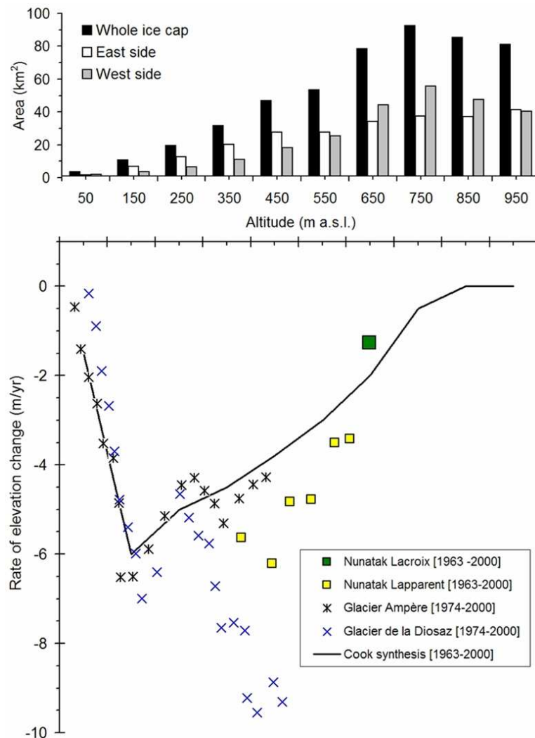
Figure 9: Hypsometry of Cook ice cap in 1963 (upper panel) and elevation changes as a function of altitude on different regions of the ice cap (lower panel). The elevation differences were measured by comparing two topographies (1974-2000, Figure 6) and analyzing the growth of nunataks (1963-2000, Figure 7).
