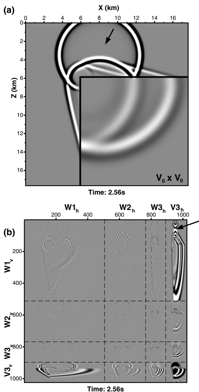
Figure 8. Corner-edge simulation. (a) Snapshot at t=2.56 \text{ s} in V_0 space. (b) Snapshot at t=2.56 \text{ s} in the wavelet domain. The arrows point to numerical pollution resulting from reflections on the horizontal interface. The pollution propagates in the fine-scale subdomain W_{1_v} \times V_{3_h} with a velocity of 4 \text{ km s}^{-1} . Owing to the coupling between scales, this noise can also be identified in the W_{3_v} \times V_{3_h} and V_{3_v} \times V_{3_h} , though the amplitude is much weaker.
