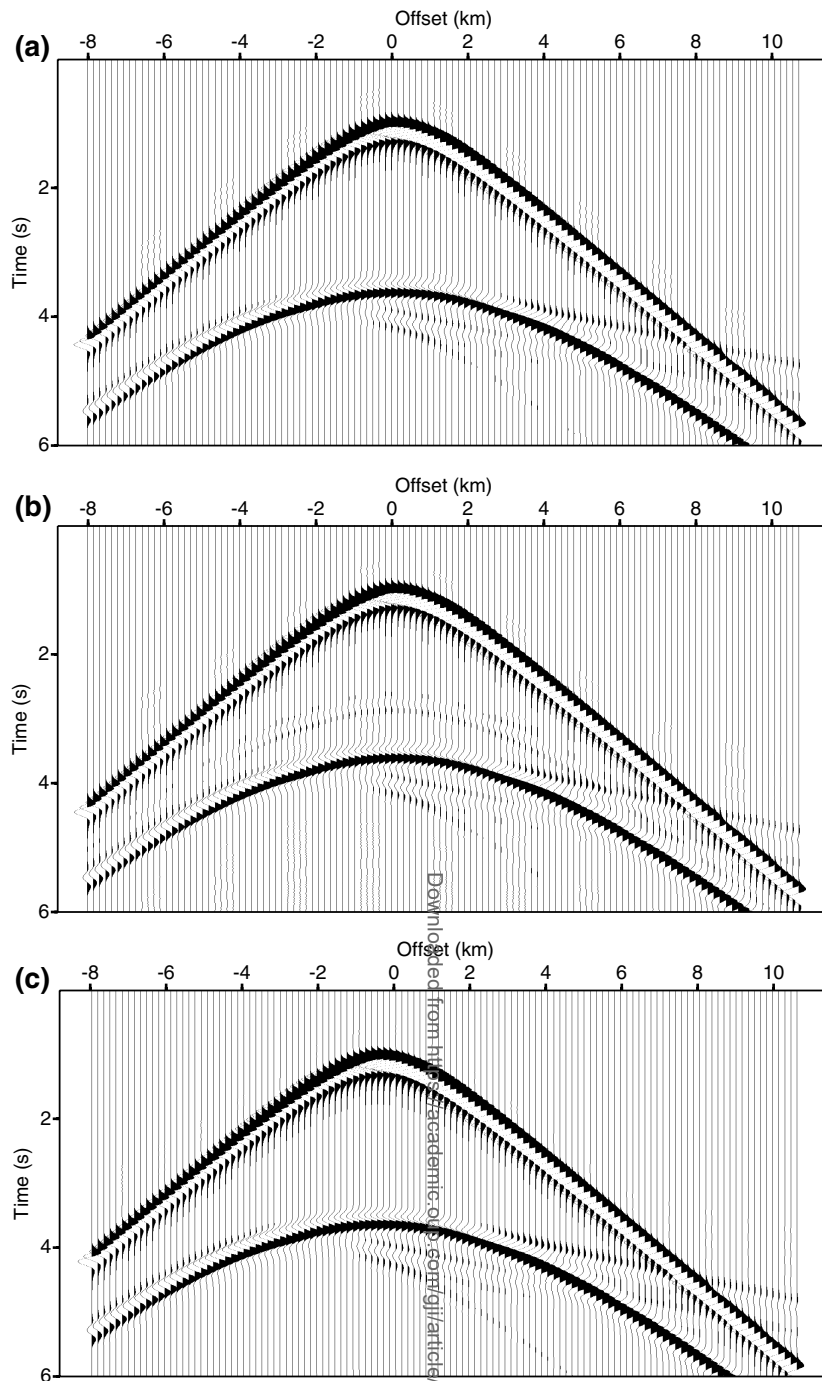
Figure 10. Corner-edge simulation. (a) Seismograms obtained with the TFD method. The receivers are located at a horizontal line at 2 km depth. (b) Seismograms extracted in the V_0 space, computed using the TPWFD method.
