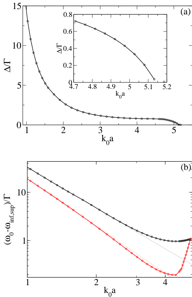
FIG. 6: (Color online) For the light spectrum in a diamond atomic lattice, in the perturbative limit \omega_p^2 \ll \omega_0^2 , and as a function of k_0a , (a) value of the omnidirectional spectral gap \Delta = \omega_{\text{sup}} - \omega_{\text{inf}} , and (b) positions of the lower frequency \omega_{\text{inf}} and upper frequency \omega_{\text{sup}} of the gap with respect to the atomic resonance frequency. a is the lattice constant (see text), k_0 = \omega_0/c and \Gamma is the spontaneous emission rate defined in (20). The inset in (a) is a magnification.
