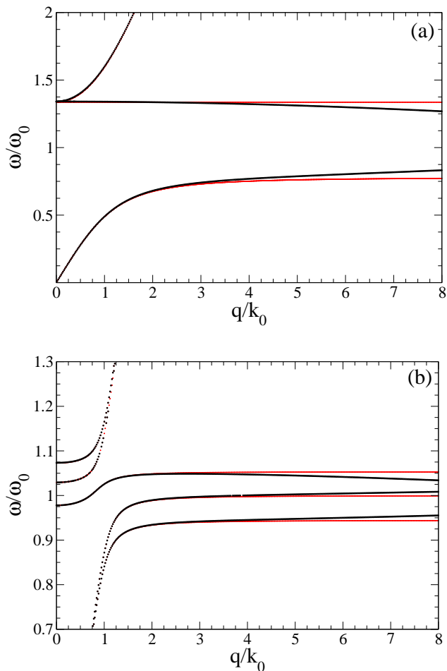
FIG. 3: (Color online) Dispersion relation for light, for the approximate long wavelength expression of Eq.(26) (red), and for the complete expression Eq.(18) (black). The spectrum is calculated as a function of q/k_0 along direction (1, 1, 1) in reciprocal space. In (a) the simple cubic lattice with k_0 a = 1/5 and \Gamma/\omega_0 = 5 \times 10^{-4} , where a is the lattice constant. The long wavelength approximation fails when the horizontal (degenerate) branches of the exact spectrum start approaching each other, eventually closing the gap at larger values of q/k_0 . In (b) an orthorhombic lattice with basis vectors in the direct space along x, y, z with norms respectively proportional to 2\pi , \pi , and 2^{3/2}\pi ; here k_0 a = 1/5 and \Gamma/\omega_0 = 5 \times 10^{-5} , where a = \mathcal{V}_L^{1/3} and \mathcal{V}_L is the volume of the primitive unit cell. Five non-degenerate branches are present, and the long wavelength approximation fails when the three horizontal branches of the exact spectrum start approaching each other, eventually closing the gap at larger values of q/k_0 .
