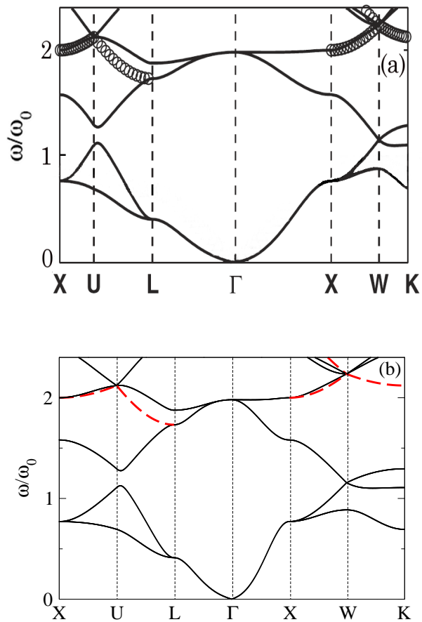
FIG. 2: (Color online) Dispersion relation for light in a fcc atomic lattice, with k_0 a \approx 3.14 , \Gamma/\omega_0 \approx 1.189 , where a is the lattice constant. (a) is the prediction found in figure (2) of [8] [circles correspond to the free modes, i.e. modes of the free field that vanish at all atomic positions], (b) is the result of calculations using Eq.(18) of this paper [the red-dashed lines correspond to the free modes]. (a) and (b) appear to be identical.
