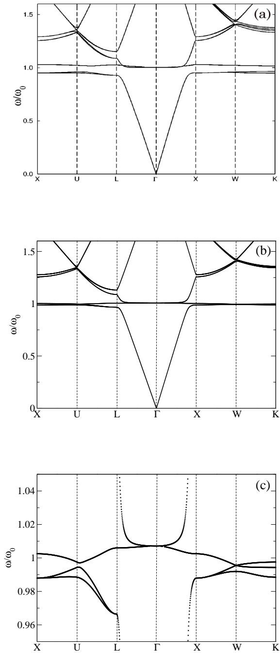
FIG. 1: Dispersion relation for light in a fcc atomic lattice, with k_0 a \approx 5 , \Gamma/\omega_0 \approx 0.0167 , where a is the lattice constant and \Gamma the spontaneous emission rate defined in (20). In (a) the prediction found in figure (1) of [7], in (b) the results of calculations obtained using Eq.(18) of this paper, and (c) is a zoom of (b) around the atomic resonance frequency. (b) and (c) show the absence of an omnidirectional photonic gap, in contradiction with (a).
