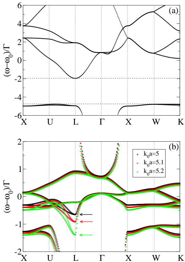
FIG. 4: (Color online) Dispersion relation for light in a diamond atomic lattice as a function of the Bloch vector along the standard irreducible path in the first Brillouin zone, in the perturbative regime \omega_p^2/\omega_0^2 \ll 1 (see text). (a) k_0 a = 2 , with k_0 = \omega_0/c and a is the diamond lattice constant (see text). Symbols: numerical values of the allowed frequencies \omega . Dashed horizontal lines: lower and upper borders of the gap obtained from the full density of states (not restricting to the irreducible path). (b) For several values of k_0 a close to the vanishing of the gap: k_0 a = 5 (black symbols), k_0 a = 5.1 (red symbols), k_0 a = 5.2 (green symbols).
