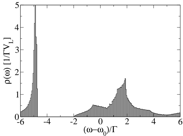
FIG. 5: Density of states \rho(\omega) for light in an diamond atomic lattice, in the perturbative regime \omega_p^2/\omega_0^2 \ll 1 , see (34). The whole unit cell of the reciprocal lattice is explored to obtain this density of states, with a mesh of 10^6 points. The histogram (with 250 bins) clearly reveals the existence of an omnidirectional gap at frequencies below the atomic resonance frequency. We have taken k_0 a = 2 as in Fig.4a. \rho(\omega) is in units of 1/(\Gamma\mathcal{V}_L) where \Gamma is the single atom spontaneous emission rate and \mathcal{V}_L = a^3/4 is the volume of the unit cell of the fcc lattice.
