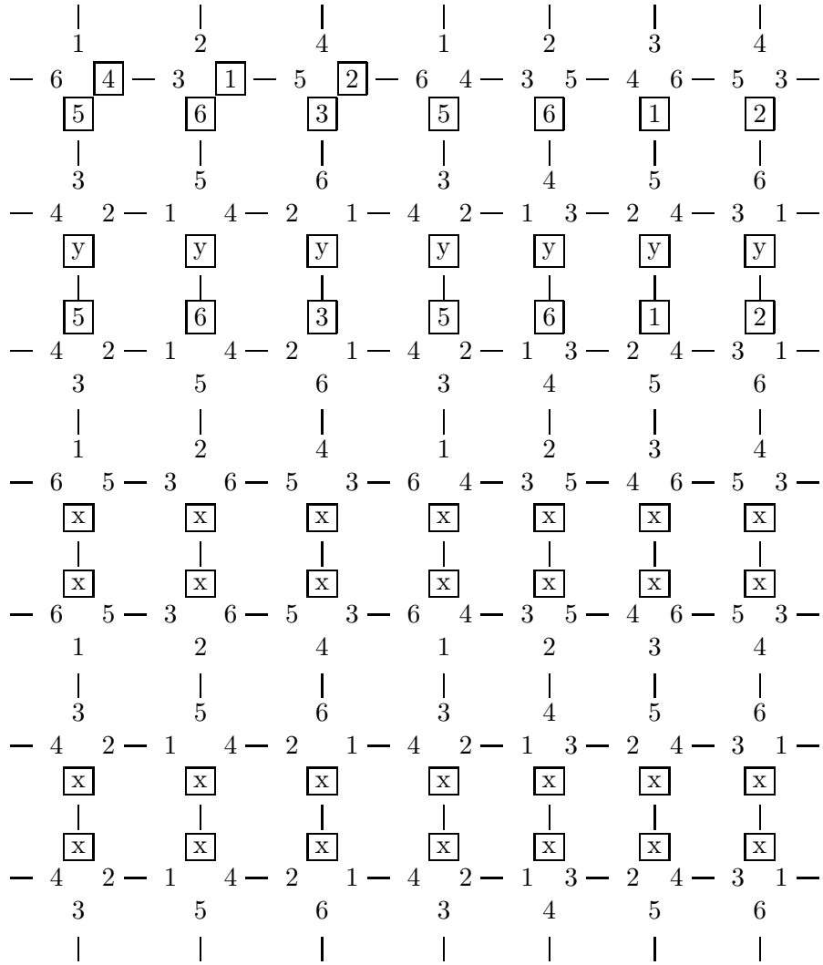
Figure 9: A partial incidence 6-coloring of T_{7,7}
