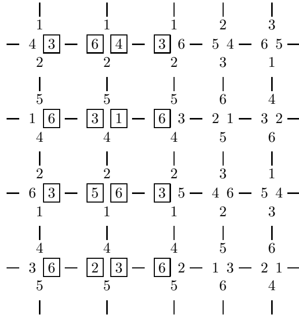
Figure 10: An incidence 6-coloring of T_{4,5}
