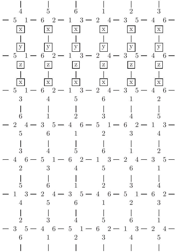
Figure 7: A partial incidence coloring of T_{7,6} .
