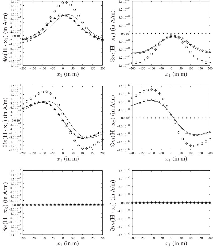
FIG. 2. Real and imaginary parts of the exact magnetic field scattered by a sphere (o), of the approximated LF one \mathbf{H}_0 (•), \mathbf{H}_0 + \mathbf{H}_2(jk)^2 (···), \mathbf{H}_0 + \mathbf{H}_2(jk)^2 + \mathbf{H}_3(jk)^3 ( \Delta ) and of the FE one (—) scattered by an ellipsoid
