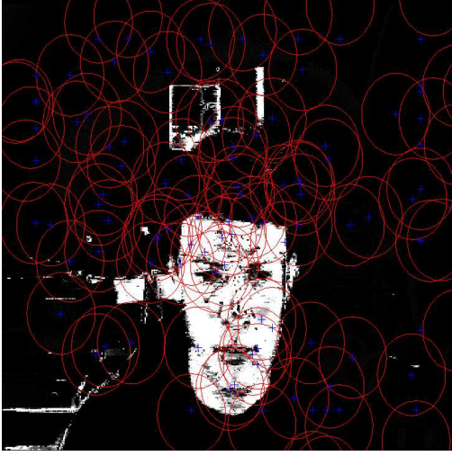
Figure 9: Particle initialisation
