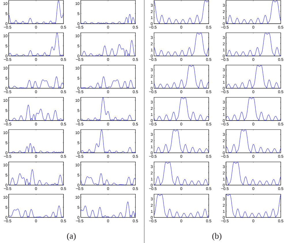
Fig. 5. Second example (in the MCLT case with window h_{a_1} ): frequency responses of synthesis filters (a) before and (b) after optimization with the cost function \tilde{J}_t .
