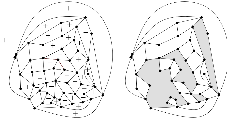
Figure 4: An Ising (or percolation) configuration and the associated exterior gasket
