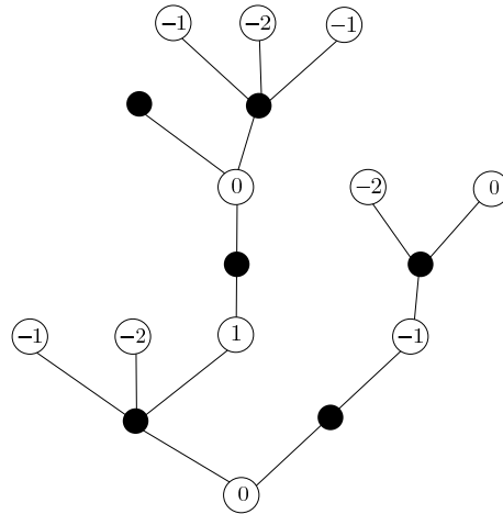
Figure 1: A rooted mobile
