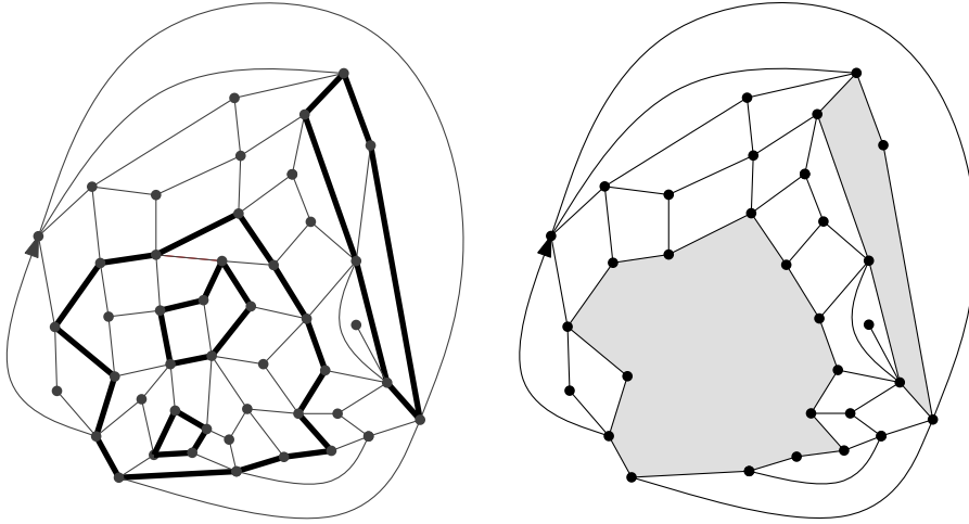
Figure 3: An O(N) configuration on a rooted quadrangulation, with 4 cycles of total length 30, and the external gasket associated with this configuration, with shaded holes of degrees 6 and 14
