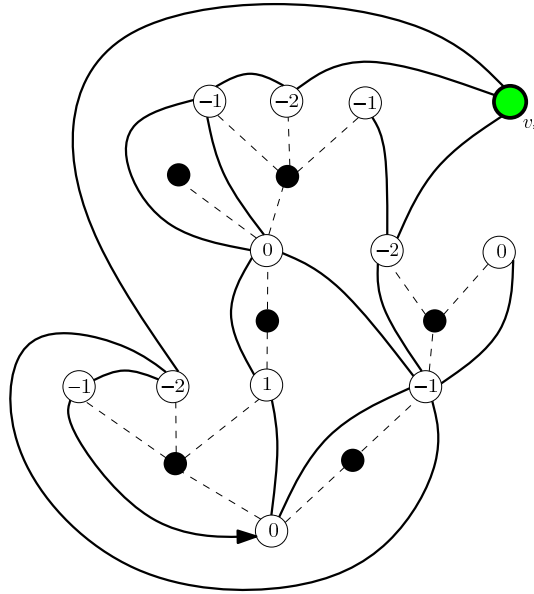
Figure 2: The Bouttier-Di Francesco-Guitter construction for the mobile of Figure 1
