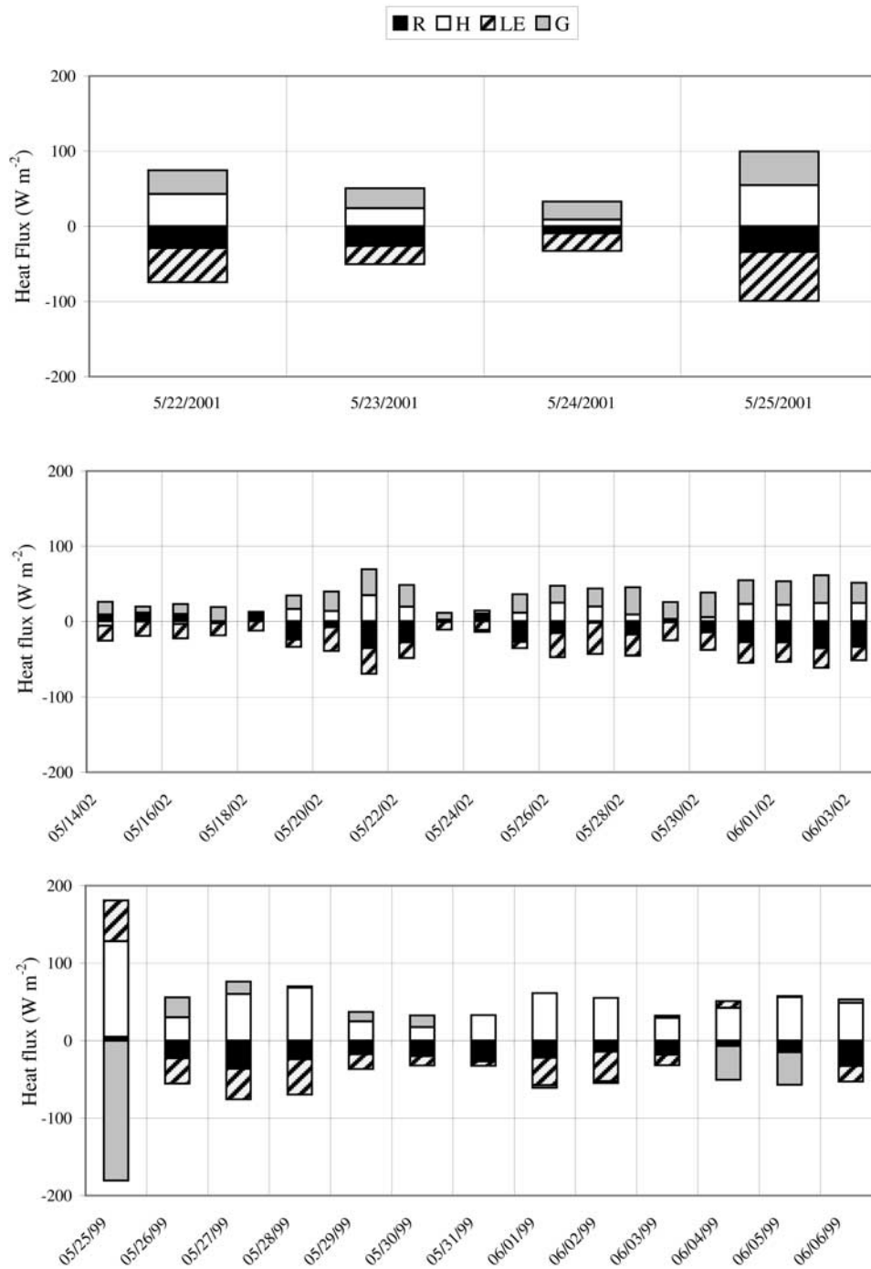
Figure 7. Daily mean values of the energy balance terms during the 2001 measuring period (upper panel), the 2002 measuring period (middle panel) and the 1999 measuring period (lower panel). The net radiation is indicated by black areas, sensible heat flux by white areas, latent heat flux by hatched areas, and the total subsurface energy flux by gray areas.
