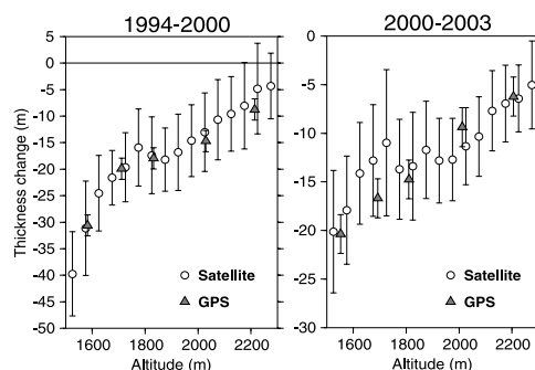
Figure 3. Comparison of the thickness change extracted from satellite images (circles) and deduced from topographic (traditional or DGPS) measurements (triangles). The left panel shows the thickness change for the 1994–2000 time interval, the right panel for 2000–2003.
