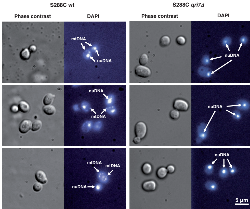
Figure 2. DAPI staining of wild-type and qri7Δ S. cerevisiae cells. Yeast strains S288C (wild-type) and S288C qri7Δ were observed under phase contrast (left panels) and after DAPI staining (right panels). mtDNA: mitochondrial DNA, nuDNA: nuclear DNA.
