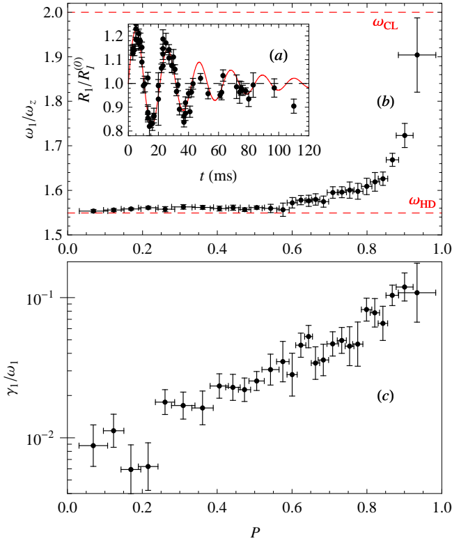
FIG. 2: (a) Oscillations of the axial radius of the majority component, for a population imbalance P = 0.85(2) , beyond the Clogston limit. The full line corresponds to a fit by an exponentially damped sinusoid. (b) Frequency of the breathing mode \omega_1 normalized to the axial trapping frequency \omega_z . The superfluid (resp. collisionless) limits \omega_1 = \sqrt{12/5}\omega_z (resp. 2\omega_z ) are indicated by the red lines. The axial (radial) trap frequency is 28.9(1) Hz ( 420 Hz). (c) Damping rate \gamma_1 as the function of polarization (in log scale). Note that our data are limited to P < 0.95 due to the small minority atom number ( N_2 \lesssim 2 \times 10^3 ) at such high polarizations.
