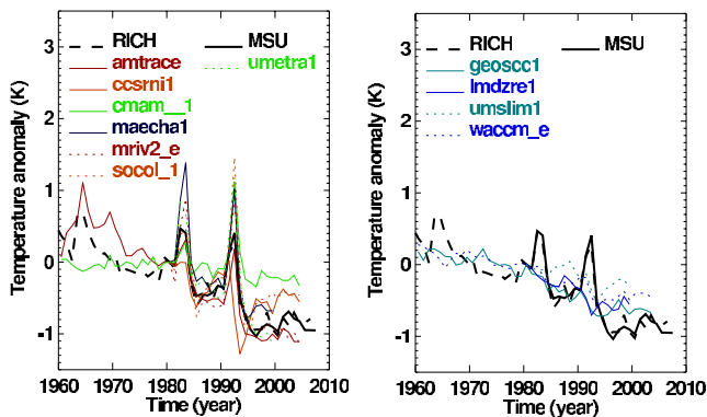
Figure 2. Global, annually averaged temperature time series, weighted in the vertical with the MSU4 channel weighting function. The values derived from the RICH radiosonde data [Haimberger et al. , 2008] are indicated by the thick broken black line. See Randel et al. [2009] for a comparison with other radiosonde datasets. MSU data are given by the bold black line. The plotted values are anomalies relative to the 1980 mean, applied individually to each data source. (left) Those models (7) which contain volcanic aerosol heating. (right) Those models (4) which exclude heating from this source.
