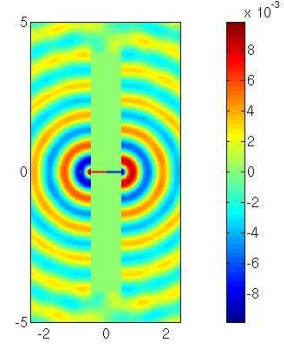
Resonant, \varepsilon = 10^{-2}
