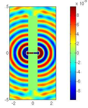
Resonant, \varepsilon = 10^{-1}
