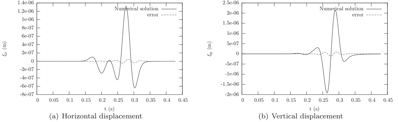
FIGURE 2. Displacement at the surface, 300 m from source, with \Delta x = 5 m, \Delta y = 5 m (10 points per wave length).
