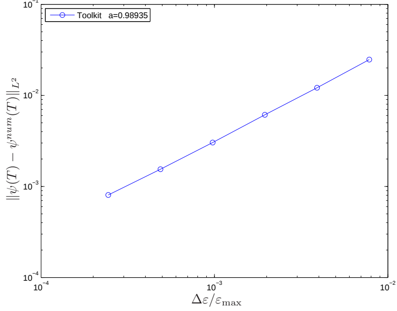
FIGURE 2. Error with respect to \Delta\epsilon , when \Delta t is small. Here, \psi^{\text{num}} stands for the approximation of \psi when using the “toolkit” method.
