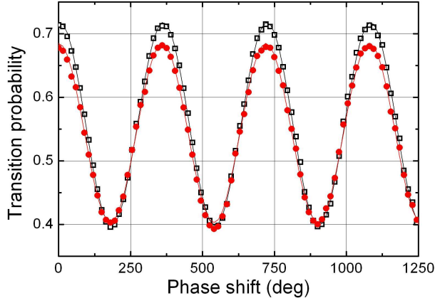
FIG. 5: (Color online) Atomic fringe patterns obtained for the interferometers A (black squares) and B (red dots) with an interaction time of 2T = 80 ms and a pulse duration of 13 \mu\text{s} . In order to scan the fringe patterns we incremented the effective Raman laser phase at each measurement cycle.
