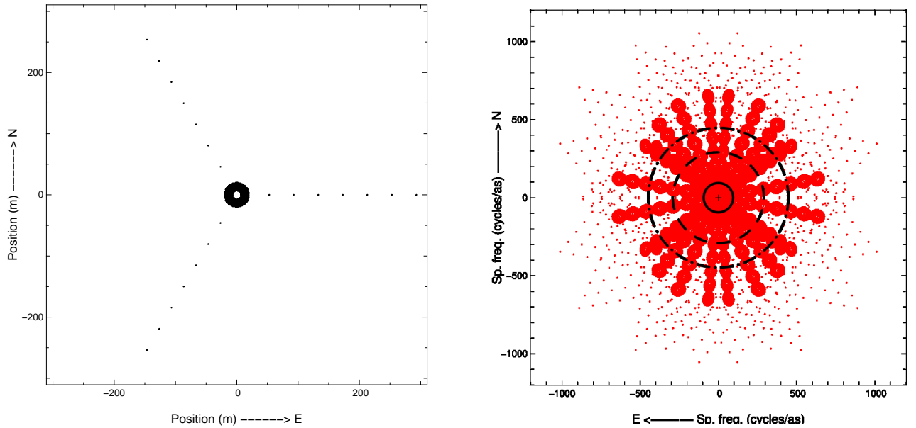
Fig. 1. A sketch of the perfect interferometer: it would combine the extreme collecting area of the E-ELT with large baselines, with a set of fixed auxilliary telescopes (ATs), made e.g. using the same segments as in the E-ELT. High fidelity images at an angular resolution of 0.45 mas in K band may be reconstructed in this configuration with only 3 different hour angles ( \approx 3 h of observing time, see UV map on the right). The center circle show the UV frequencies probed by the E-ELT alone, the dashed circle show the same for the VLTI (130 m maximum baseline) and the dash-dotted circle represent the maximum reachable baseline of the VLTI (200 m), with an upgrade of its delay lines.
