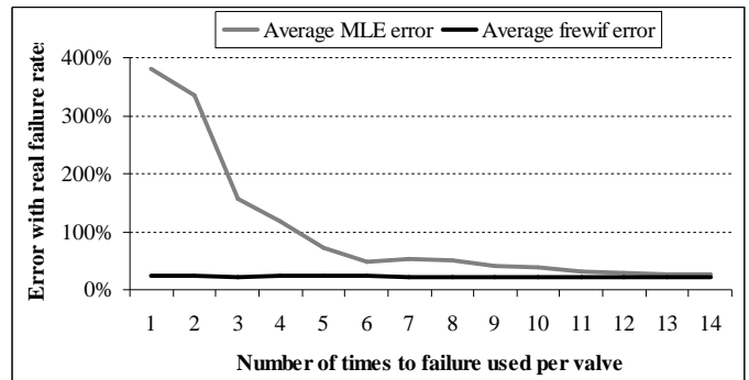
Figure 9. Average percentage of error with the real failure rates, according to the number of times to failure observed per valve (quantity of feedback data)
