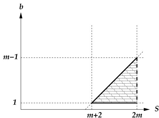
Figure 1: Parameters (b, S) for a given m .
