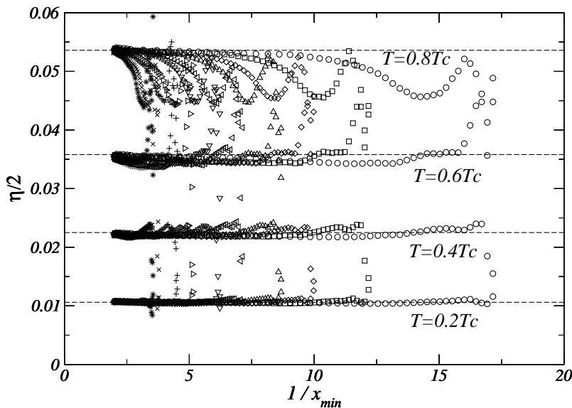
Figure 4. Effective exponent \eta/2 obtained by interpolation of the spin-spin correlation function in the aging regime. The different curves correspond to temperatures 0.2T_c , 0.4T_c , 0.6T_c and 0.8T_c (from bottom to top) and the different symbols to different waiting times s . The exponents \eta/2 obtained in the quasi-equilibrium regime are plotted as a dashed line.
