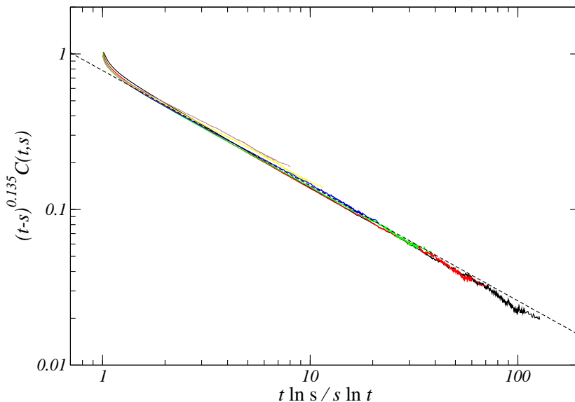
Figure 8. Scaling function (t-s)^{\eta/2}C(t,s) versus \frac{t \ln s}{s \ln t} of the spin-spin correlation function for the FFXY prepared in a random state and quenched at the critical temperature. The different curves correspond to different waiting times ( s = 500, 1000, 2000, 4000, 8000, and 12000 ). The dashed line corresponds to the power-law \left(\frac{t \ln s}{s \ln t}\right)^\phi with \phi = 0.74 .
