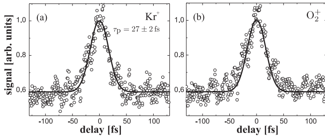
FIG. 4: Time resolved two-photon ionization trace of krypton and oxygen. Solid lines show numerical simulations: (a) \tau_p = 27 \pm 2 fs.
