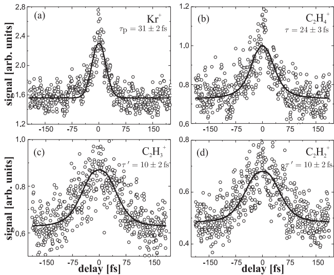
FIG. 3: Time resolved two-photon ionization trace of krypton and ethylene. Solid lines show numerical simulations: (a) \tau_p = 31 \pm 2 fs, (b) \tau_p = 31 \pm 2 fs, \tau = 24 \pm 3 fs, (c) and (d) \tau_p = 31 \pm 2 fs, \tau = 24 \pm 3 fs, and \tau' = 10 \pm 2 fs (see text). The data are normalized to the ethylene ion signal.
