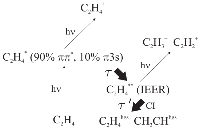
FIG. 1: Photoreaction path-network. IEER: intermediate electronically excited region; CI: conical intersection; hgs: hot ground state. Black solid arrows indicate the processes of interest in this work with \tau and \tau' the decay times of these processes.
