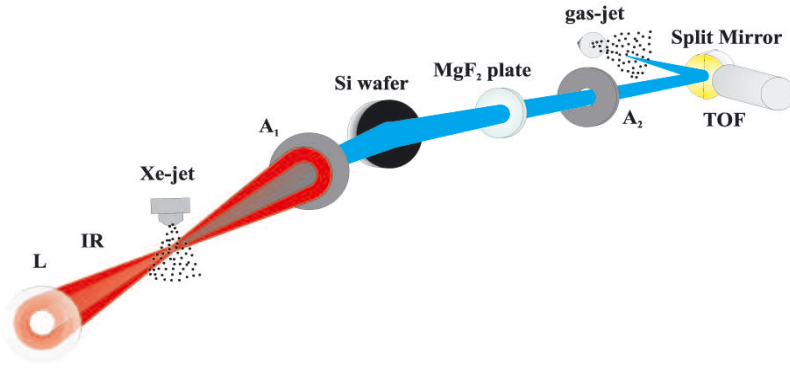
FIG. 2: Experimental setup. L: lens; A 1 : aperture, differential pumping; A 2 : aperture. The pulsed nozzle of the gas jet also serves as repeller of the TOF spectrometer.
