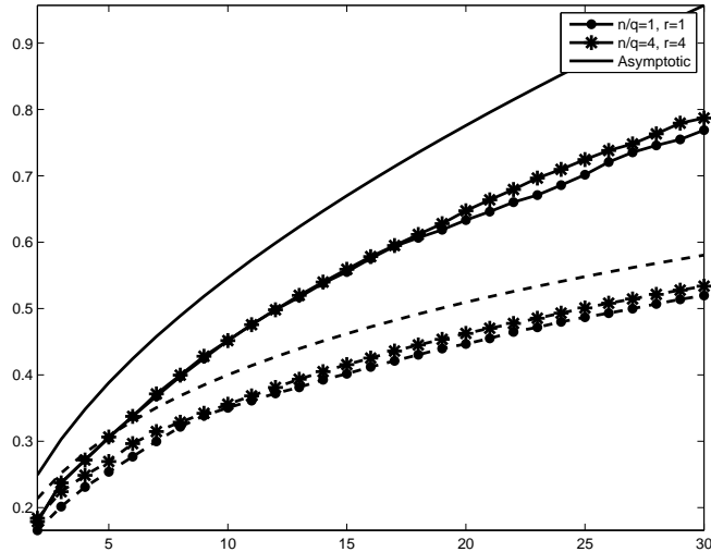
Figure 5: Comparison of the different variants of Algorithm 3-2 for (N, P) = (8000, 2000) . Solid and dashed lines correspond respectively to \tilde{\delta}_s^{\max} and \tilde{\delta}_s^{\min} . Circles: greedy pursuit Q = R = 1 . Asterisks: pruned weak greedy pursuit Q = N/4, R = 4 . The curves without circles or asterisks corresponds to the asymptotic upper bounds of [22].
