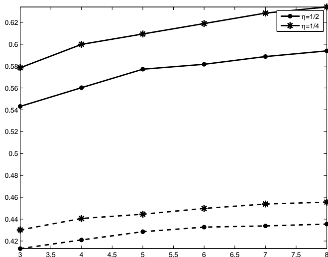
Figure 6: Plot of \tilde{\delta}_s^{\max} (solid curves) and \tilde{\delta}_s^{\min} (dashed curves) as a function of s , for two values of \eta = P/N and for P = 100s . The curves are obtained by averaging the value of \tilde{\delta}_s^{\max} and \tilde{\delta}_s^{\min} for 5 realizations of the random matrix A .
