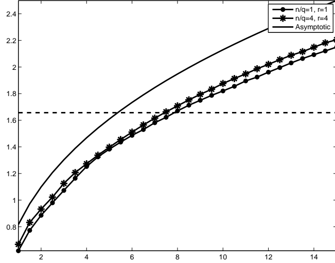
Figure 7: Display of (4\sqrt{2} - 3)\tilde{\delta}_{2s}^{\min} + \tilde{\delta}_{2s}^{\max} for (N, P) = (8000, 2000) , computed using our greedy pursuit with no pruning (circles) and pruning (asterisks, Q = N/4 ). The solid curve corresponds to the asymptotic upper bound of [22]. The dashed line corresponds to the limit y = 4(\sqrt{2} - 1) below which condition (16) is fulfilled.
